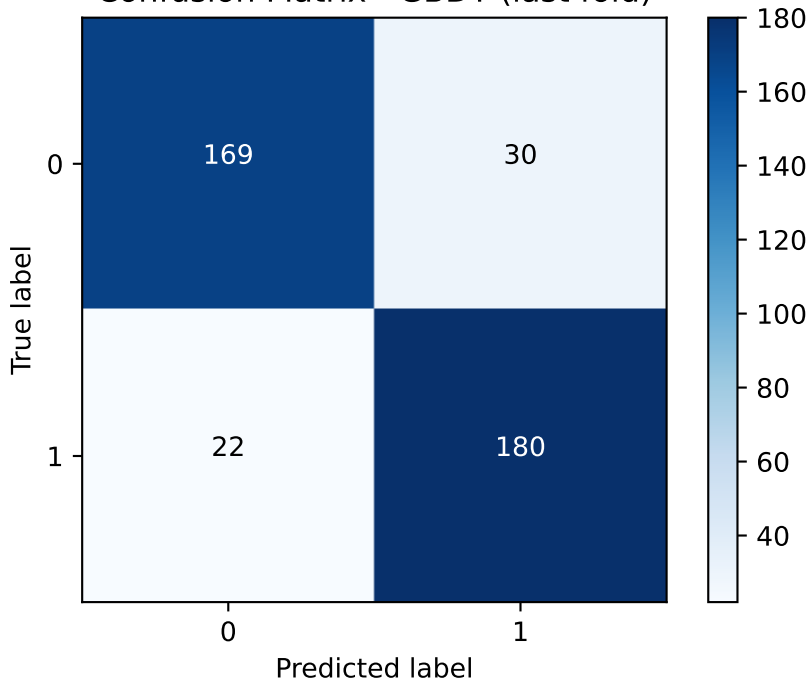
Confusion Matrix - GBDT (last fold)
