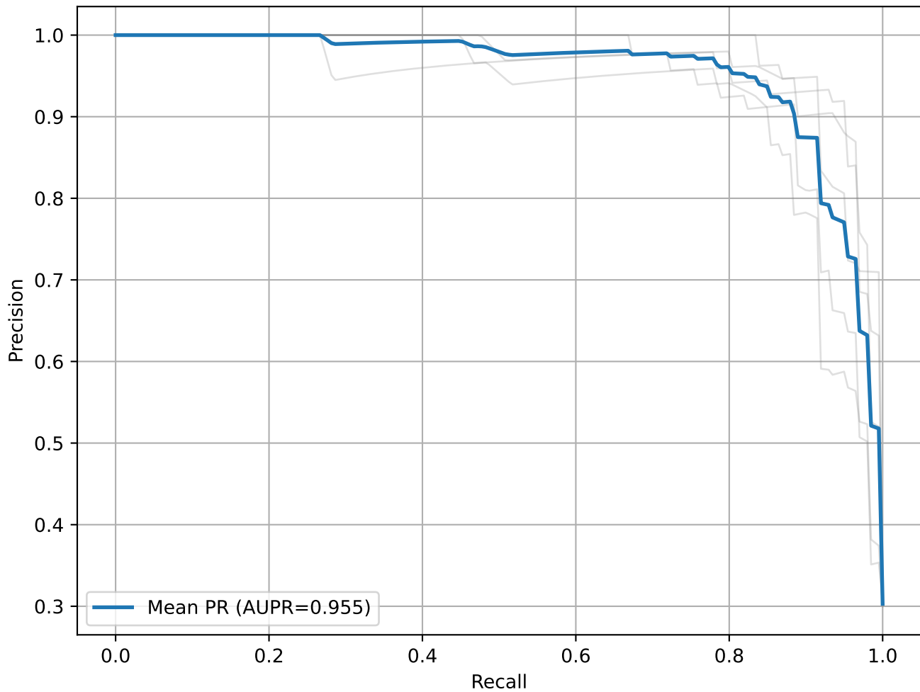
Precision-Recall - RF
