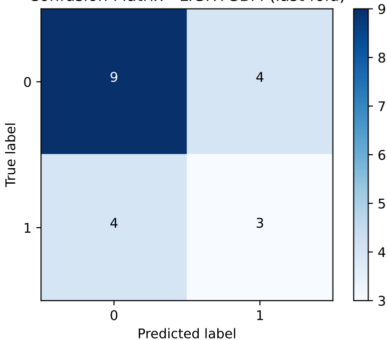
Confusion Matrix - LIGHTGBM (last fold)
