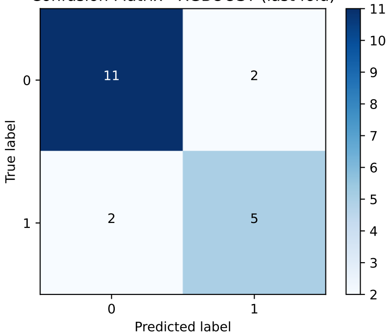
Confusion Matrix - XGBOOST (last fold)
