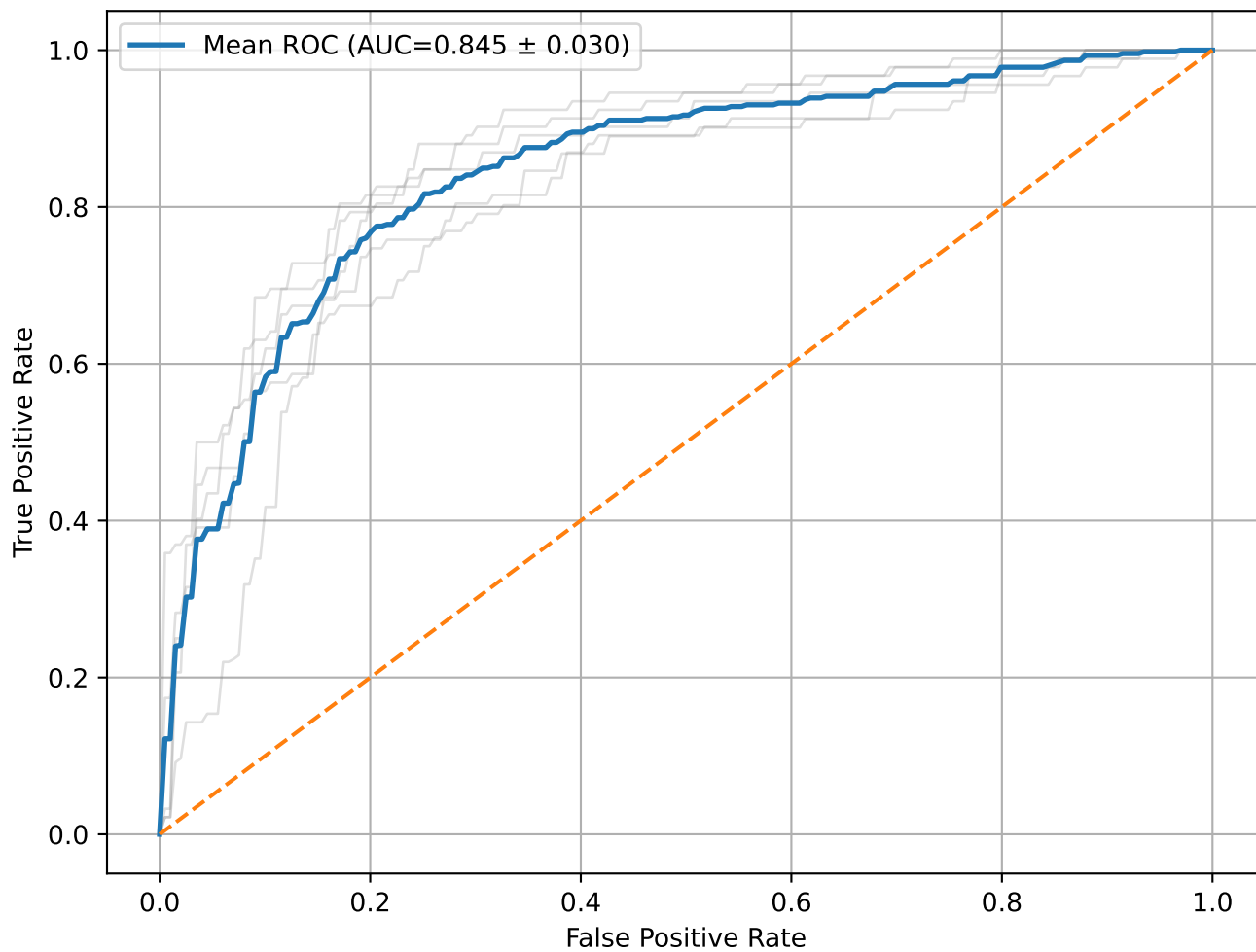
ROC - GBDT
