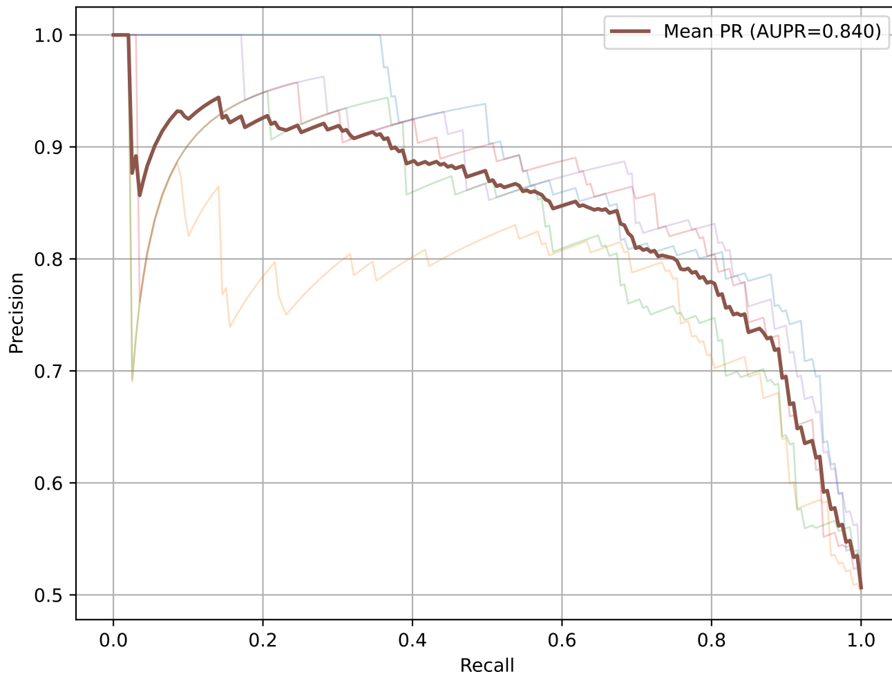
Precision-Recall - GBDT
