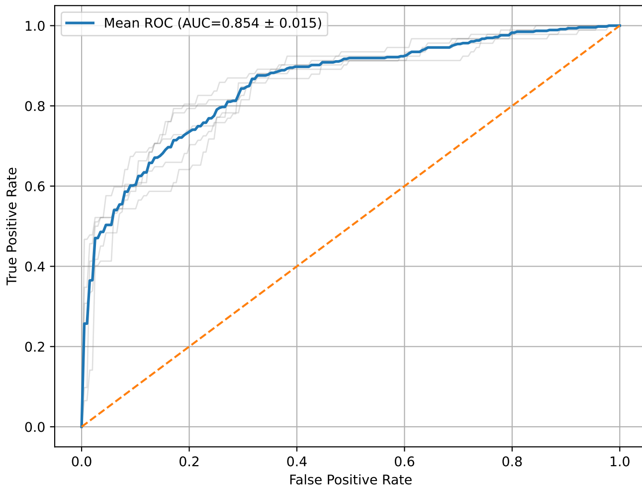
ROC - STACKING
