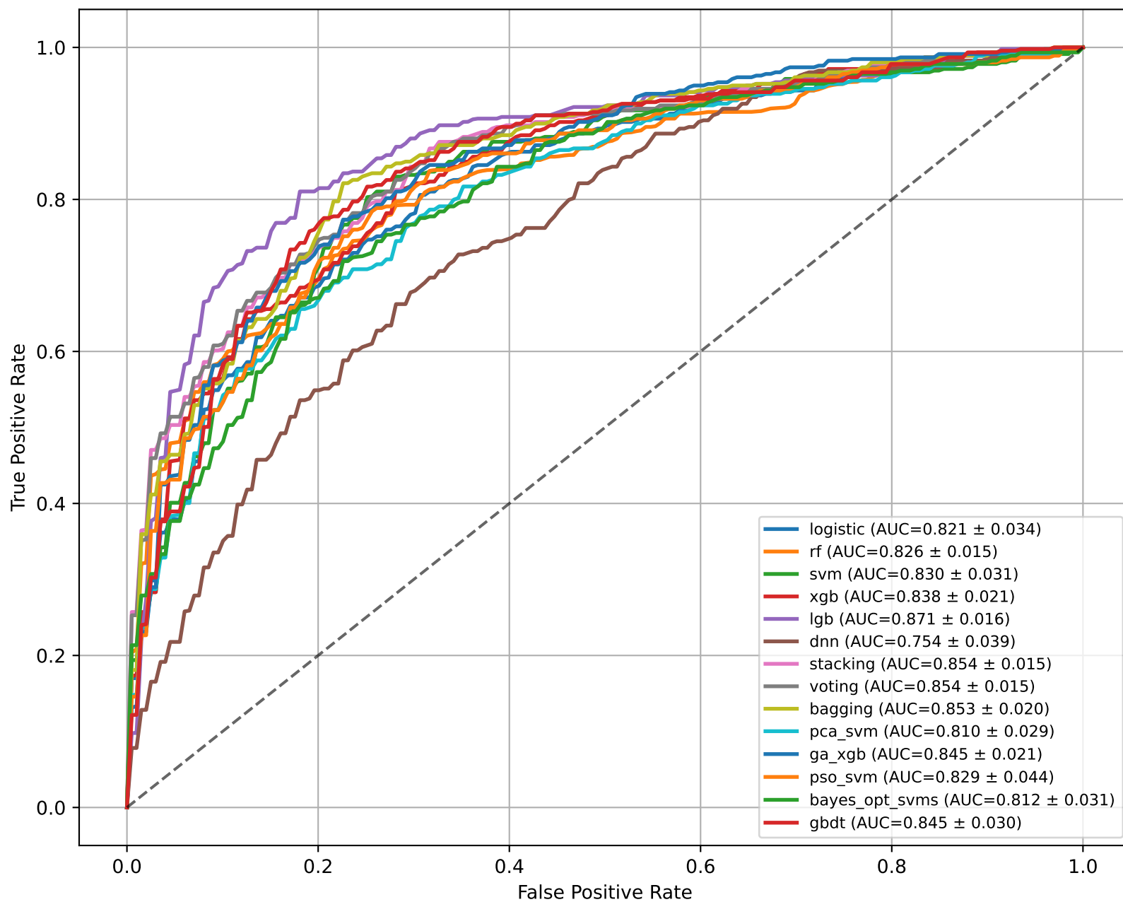
Combined ROC - All Models
