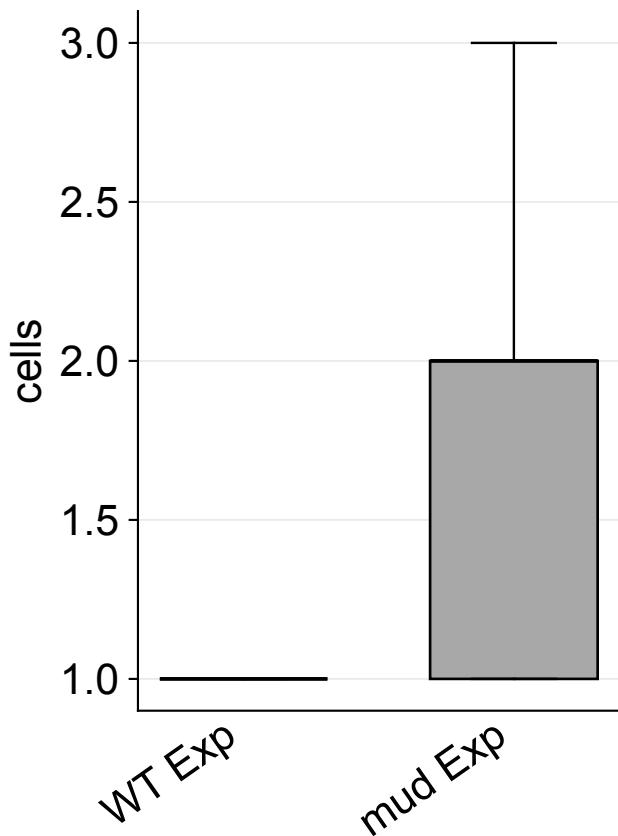
NB count
