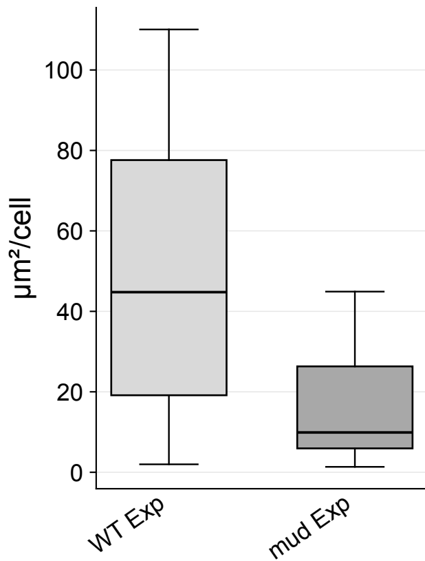
Mean NB area
