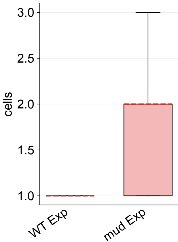
NB count
