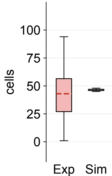
Pros count
