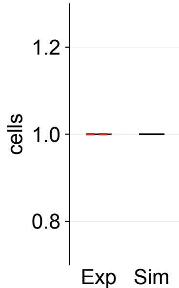
NB count
