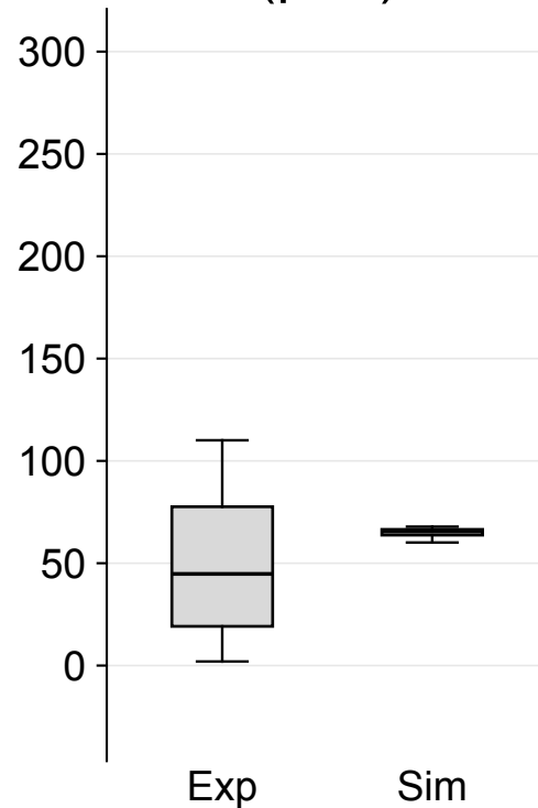
Total NB area ( \mu\text{m}^2 )
