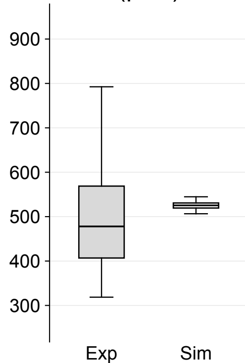
Lineage area ( \mu\text{m}^2 )
