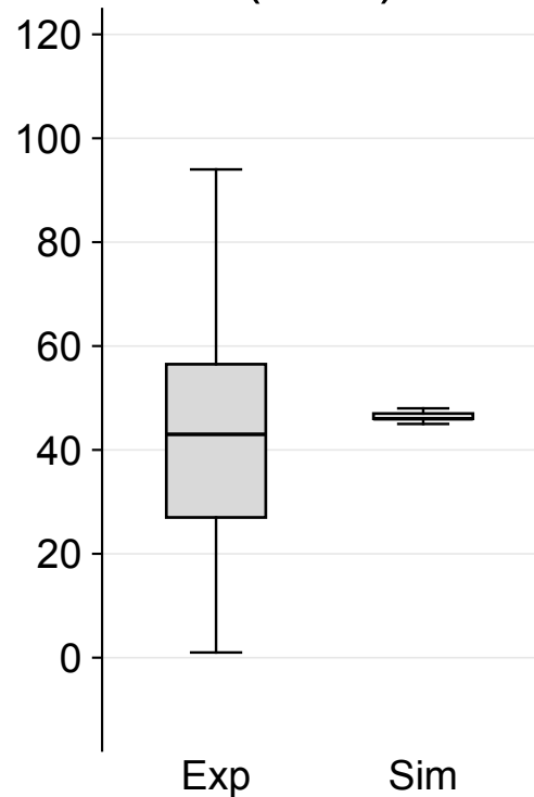
Pros count (cells)
