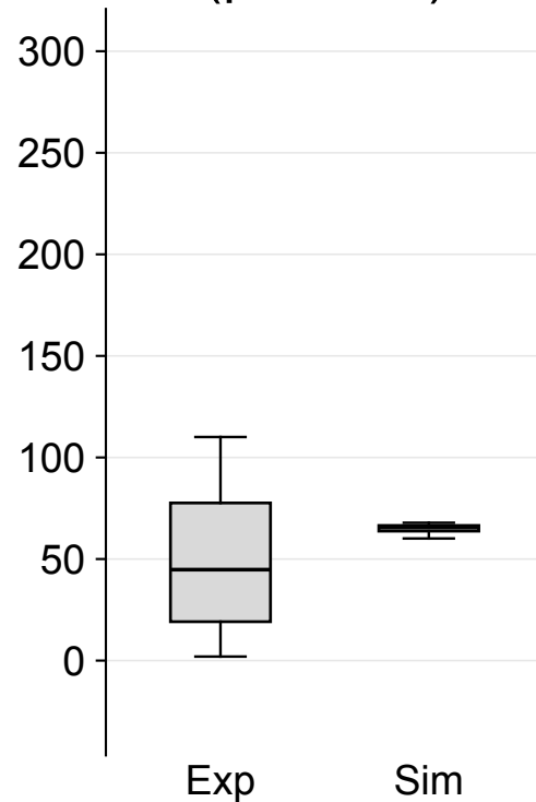
Mean NB area ( \mu\text{m}^2/\text{cell} )
