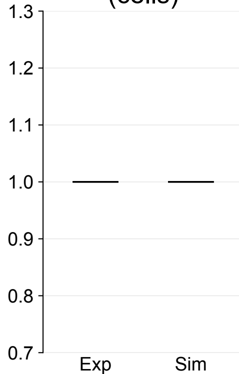
NB count (cells)
