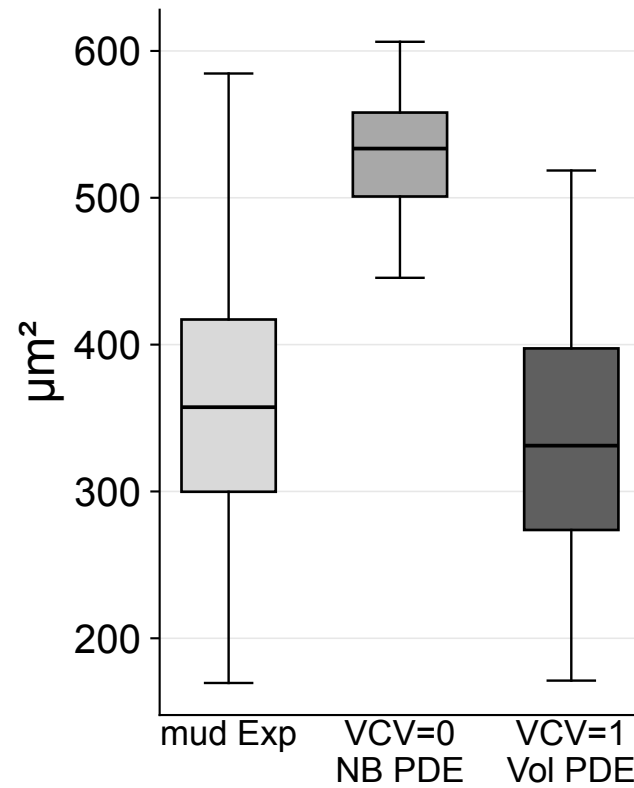
Lineage area
