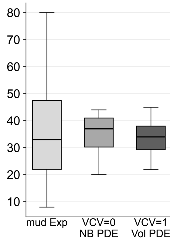
Pros count
