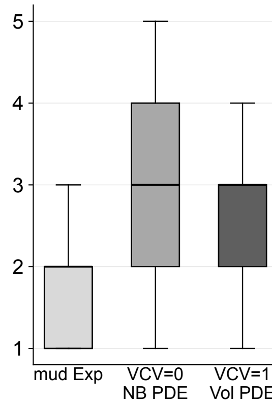
NB count
