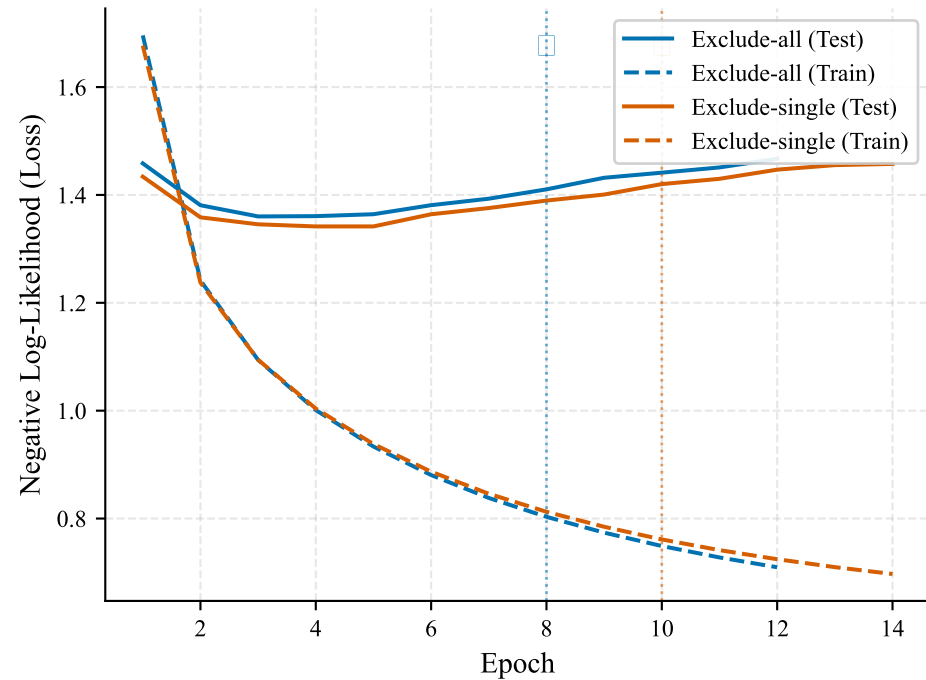
(a) Learning Curve: Loss
