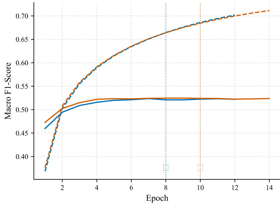
(b) Learning Curve: Macro-F1
