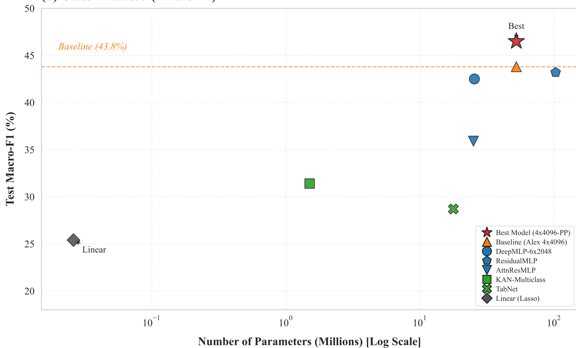
(b) Class-Balanced (Macro-F1)
