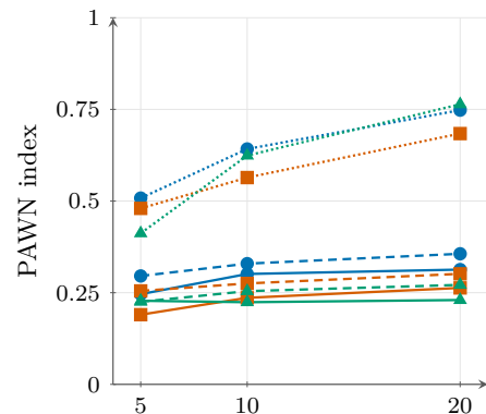
(a) p_0 = 10\%
