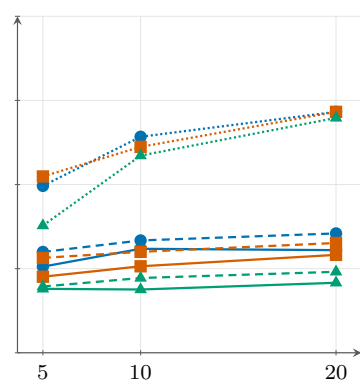
(c) p_0 = 50\%
