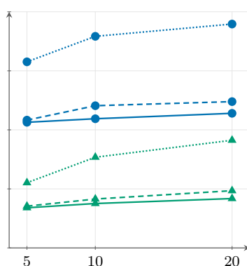
(e) p_0 = 30\%
