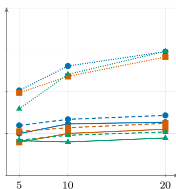
(b) p_0 = 30\%
