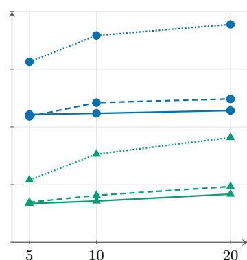
(f) p_0 = 50\%
