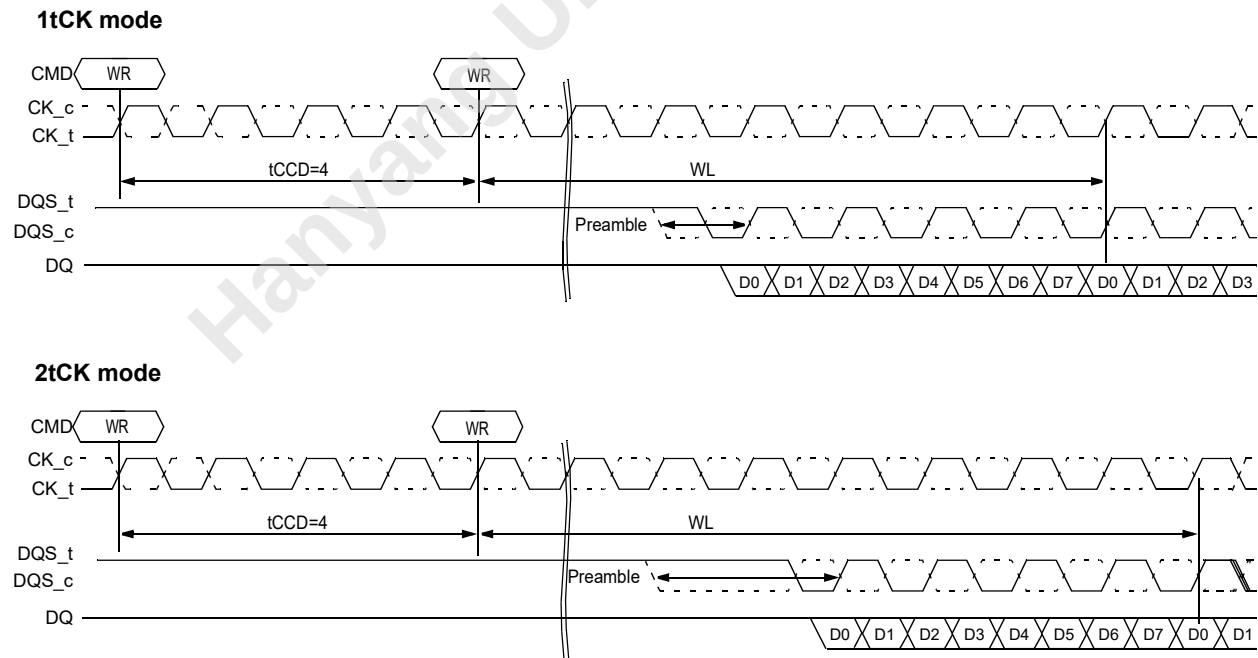
Figure 76 — tCCD=4 (AL=PL=0)
