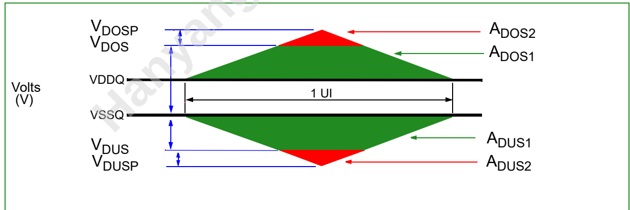
Figure 209 — Data, Strobe and Mask Overshoot and Undershoot Definition
