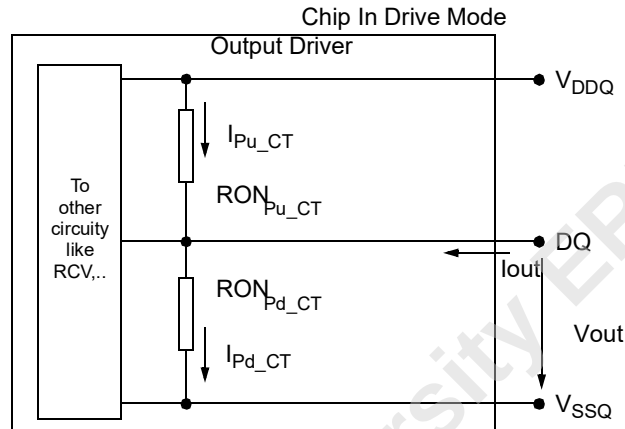
Figure 220 — Output Driver
