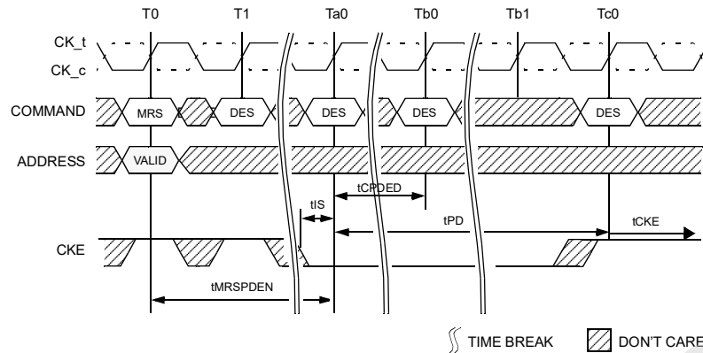
Figure 171 — MRS Command to Power-Down Entry
