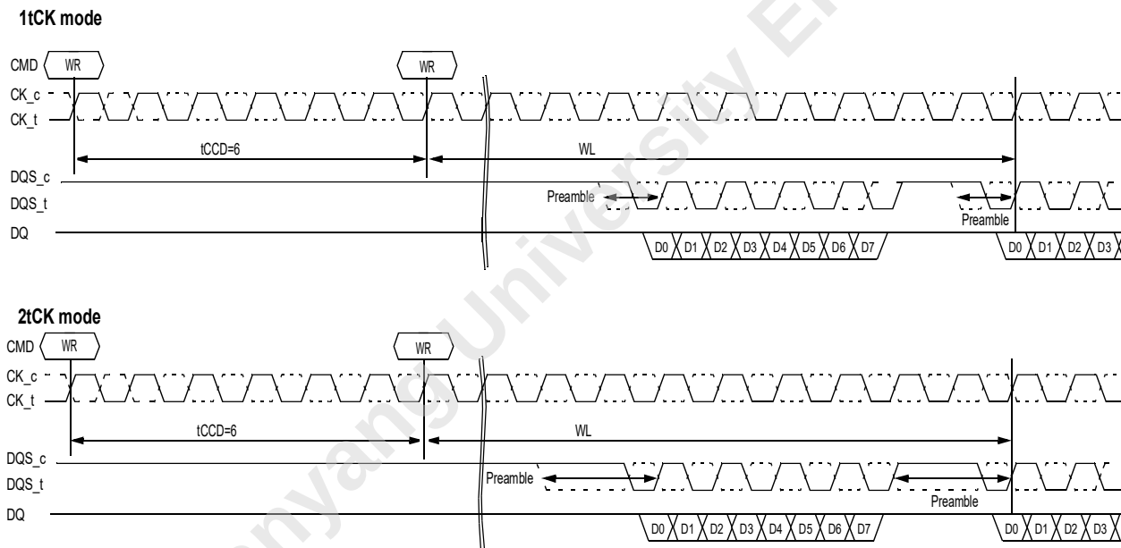
Figure 78 — tCCD=6 (AL=PL=0)
