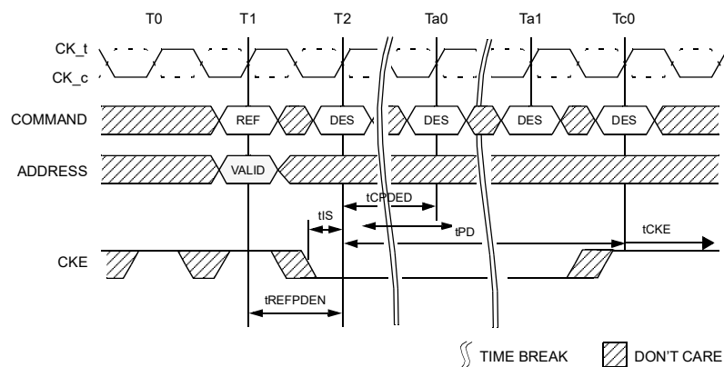
Figure 168 — Refresh Command to Power-Down Entry
