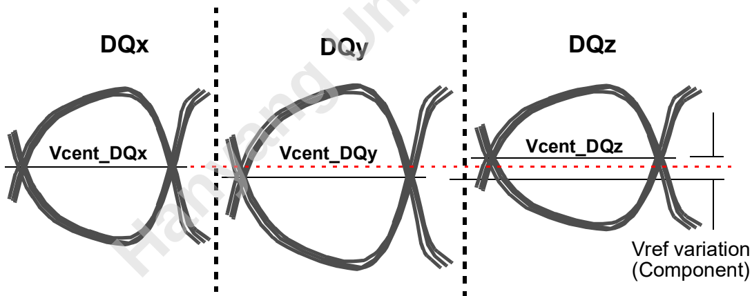
Figure 229 — Vcent_DQ Variation to Vcent_DQ(midpoint)
