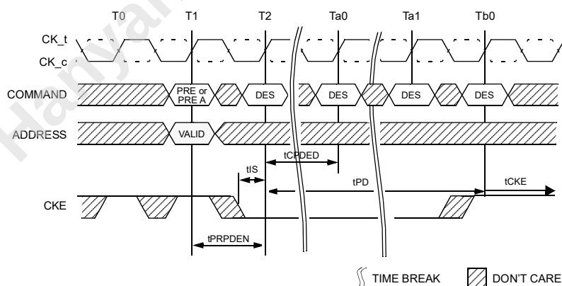
Figure 170 — Precharge/Precharge all Command to Power-Down Entry
