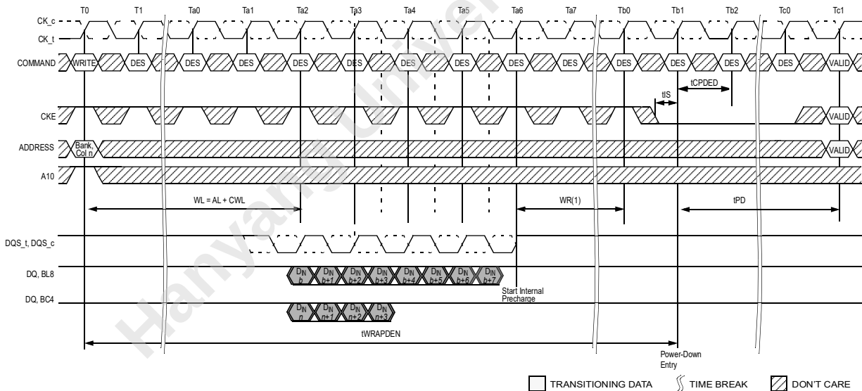
Figure 165 — Power-Down Entry After Write with Auto Precharge
