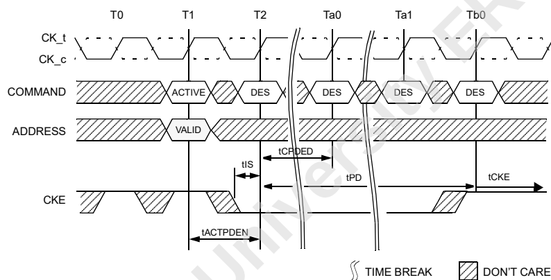
Figure 169 — Activate Command to Power-Down Entry
