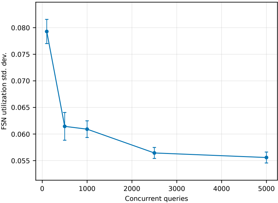
Proposed (MA-LB-PQ-VDSE)
