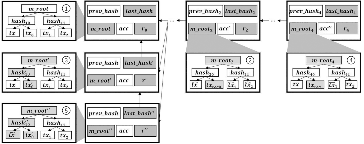
Fig. 1. An attack on Jia et al.'s redactable blockchain.
