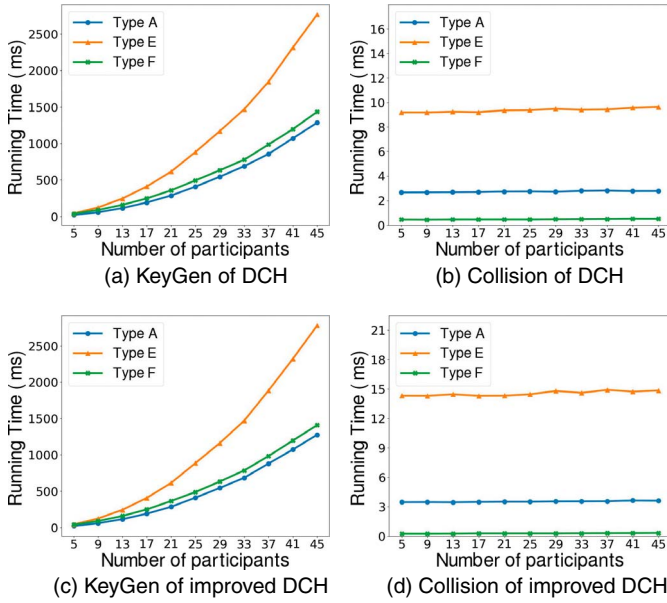
Fig. 2. Execution time analysis on the KeyGen and Collision algorithms of DCH and improved DCH under different numbers of participants based on different types of pairings.
