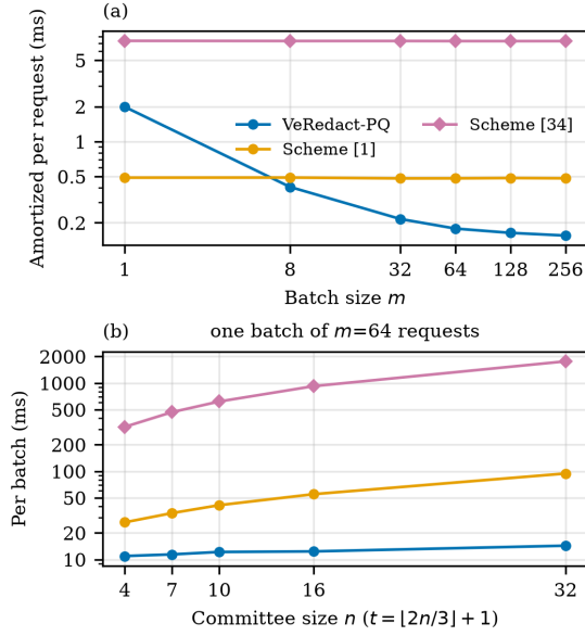
Fig. 4: Authorization latency: (a) amortized latency per request versus batch size and (b) per-batch latency versus committee size.
