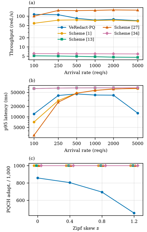
Fig. 3: Redaction performance: (a) throughput and (b) 95th-percentile end-to-end latency versus request arrival rate, and (c) PQCH adaptations per 1,000 redactions versus Zipf skew.
