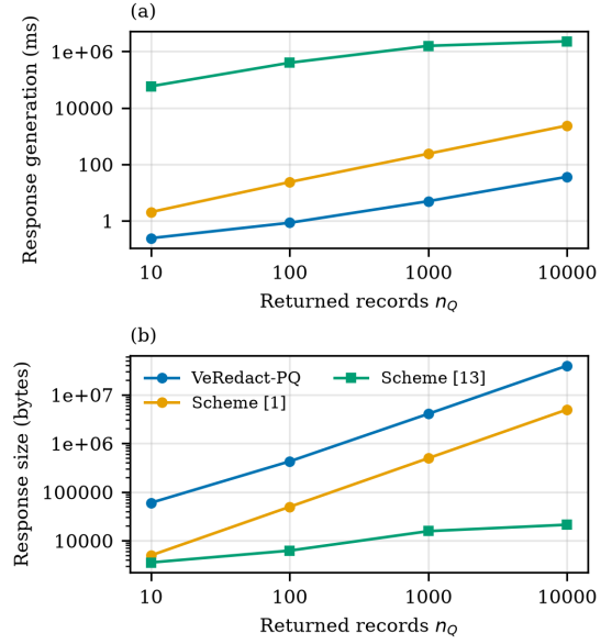
Fig. 5: Audit efficiency: (a) response-generation time and (b) audit-response size versus the number of returned records.
