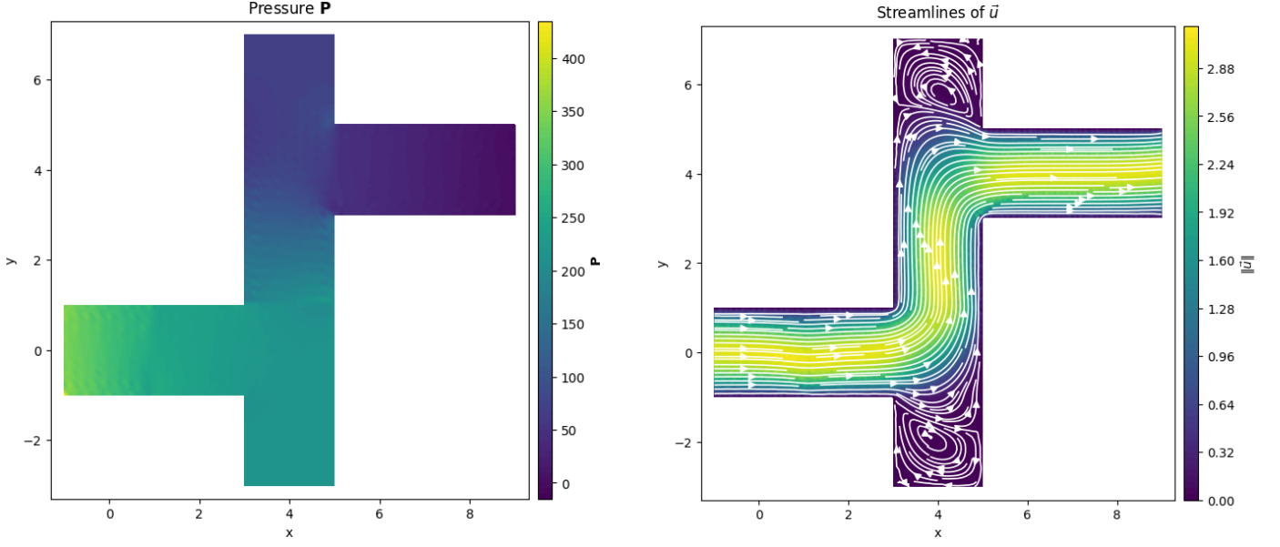
Figure 9: Complete Stokes flow simulation inside the Z-Shaped Channel Device domain.
