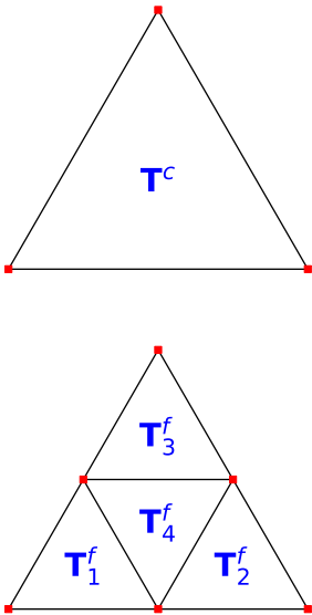
Figure 2: Macro element and its corresponding subdivision into 4 congruent elements.
