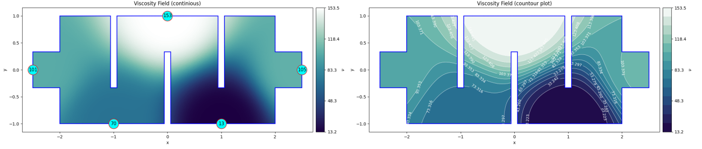
Figure 11: The viscosity field \nu(\mathbf{x}; \boldsymbol{\mu} = [101.014 \quad 70.127 \quad 153.464 \quad 13.205 \quad 104.624]^T) across the exchanger device's domain.
