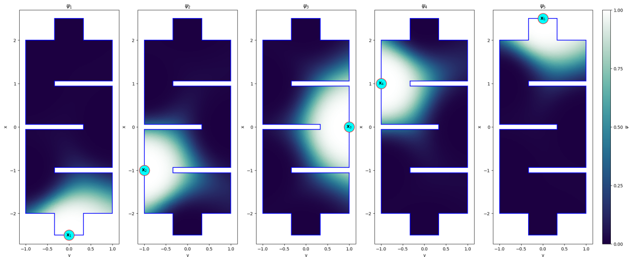
Figure 12: The viscosity basis functions \{\psi_i\}_{i=1}^5 across the exchanger device's domain.
