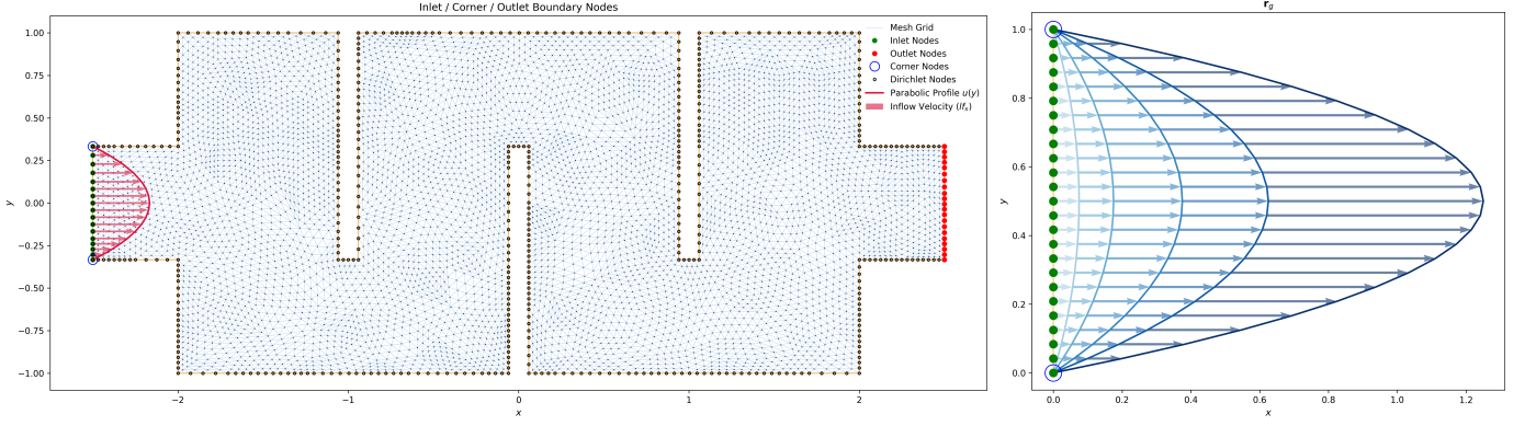
(a) Computational domain and boundary node classification. The left boundary features an inflow velocity function g_x(y) evaluated at green inlet nodes. It is important that the function remains anchored to zero at the top and bottom blue corner nodes to guarantee seamless continuity with the no-slip black Dirichlet wall nodes. The downstream outlet red boundary nodes remain unconstrained for traction-free outflow. (b) \mathbf{r}_g depicted for a set of \alpha values, namely: \alpha_i \in \{0.3, 0.7, 1.5, 2.5, 5\} .
