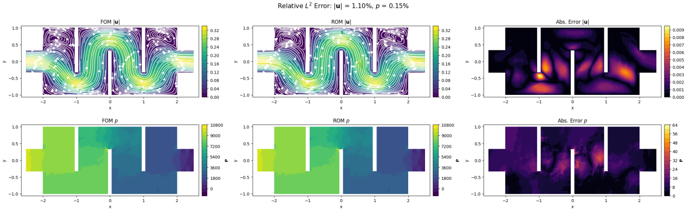
Figure 15: ROM vs FEM
