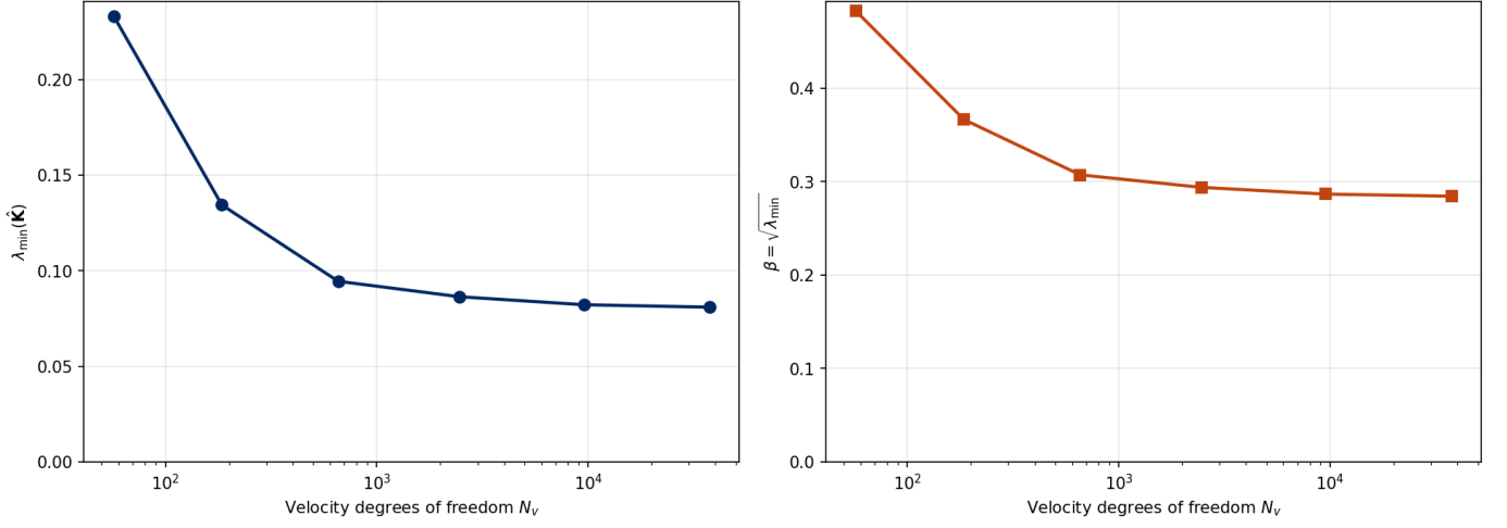
Figure 6: Discrete inf-sup eigenvalue \lambda_{\min} (left) and stability constant \beta (right) as a function of velocity degrees of freedom N_v , over six uniform refinement levels.
