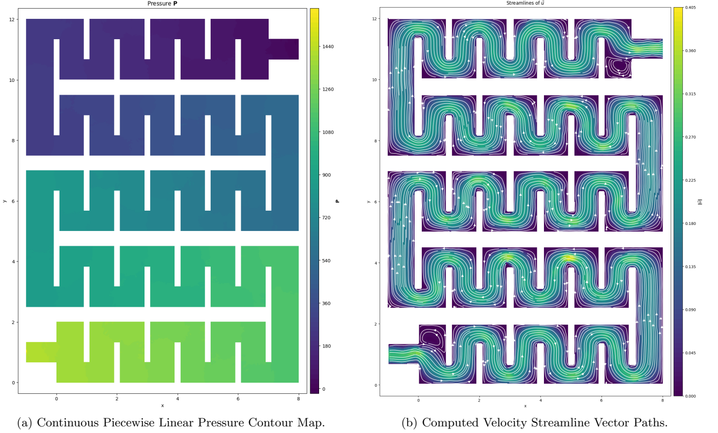
Figure 8: Complete Stokes flow simulation inside the Winding Pipe domain.
