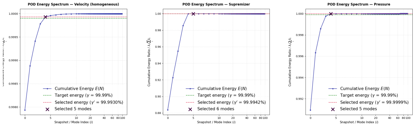
Figure 14: Cumulative POD energy spectra E(N) and target truncation thresholds (\gamma) for the velocity, supremizer, and pressure snapshot spaces.
