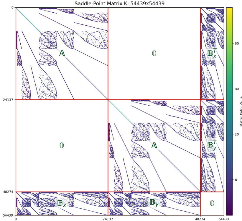
Figure 5: A matrix constructed for the exchanger device's geometry.
