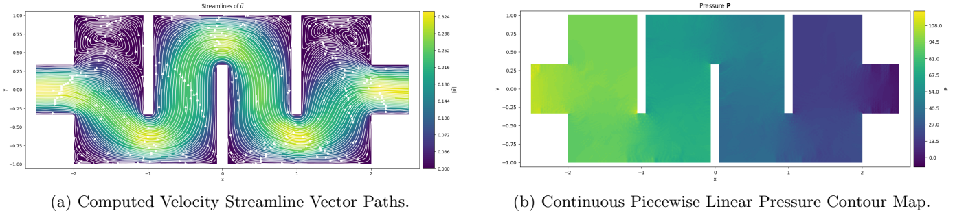
Figure 7: Complete Stokes flow simulation inside the Exchanger Device domain.
