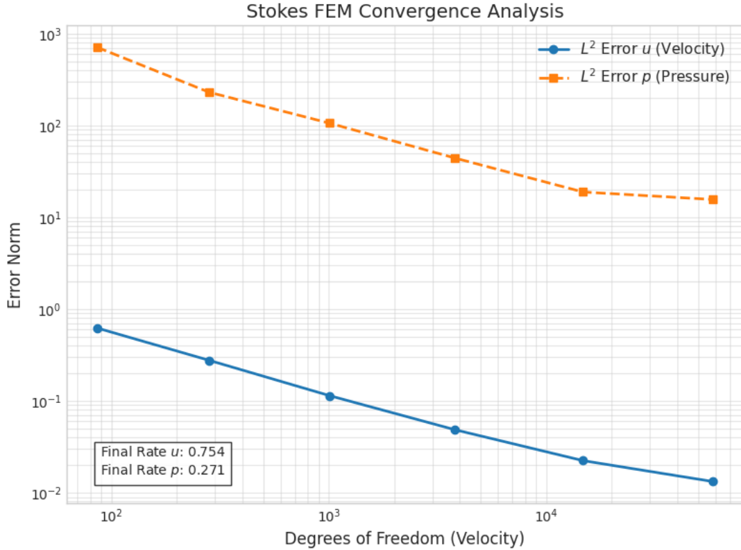
Figure 10: Log-log plot of the L^2 error norms for velocity and pressure against the velocity degrees of freedom.
