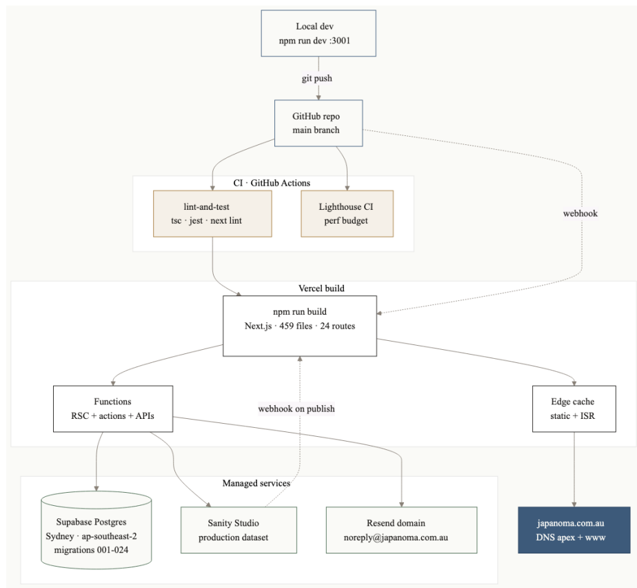
Deployment topology
