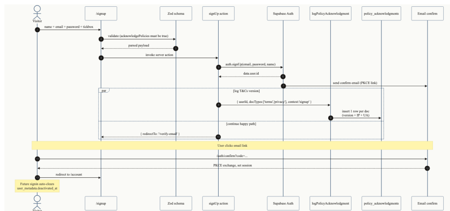
Auth and signup flow
