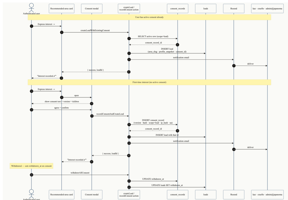
Lead capture flow
