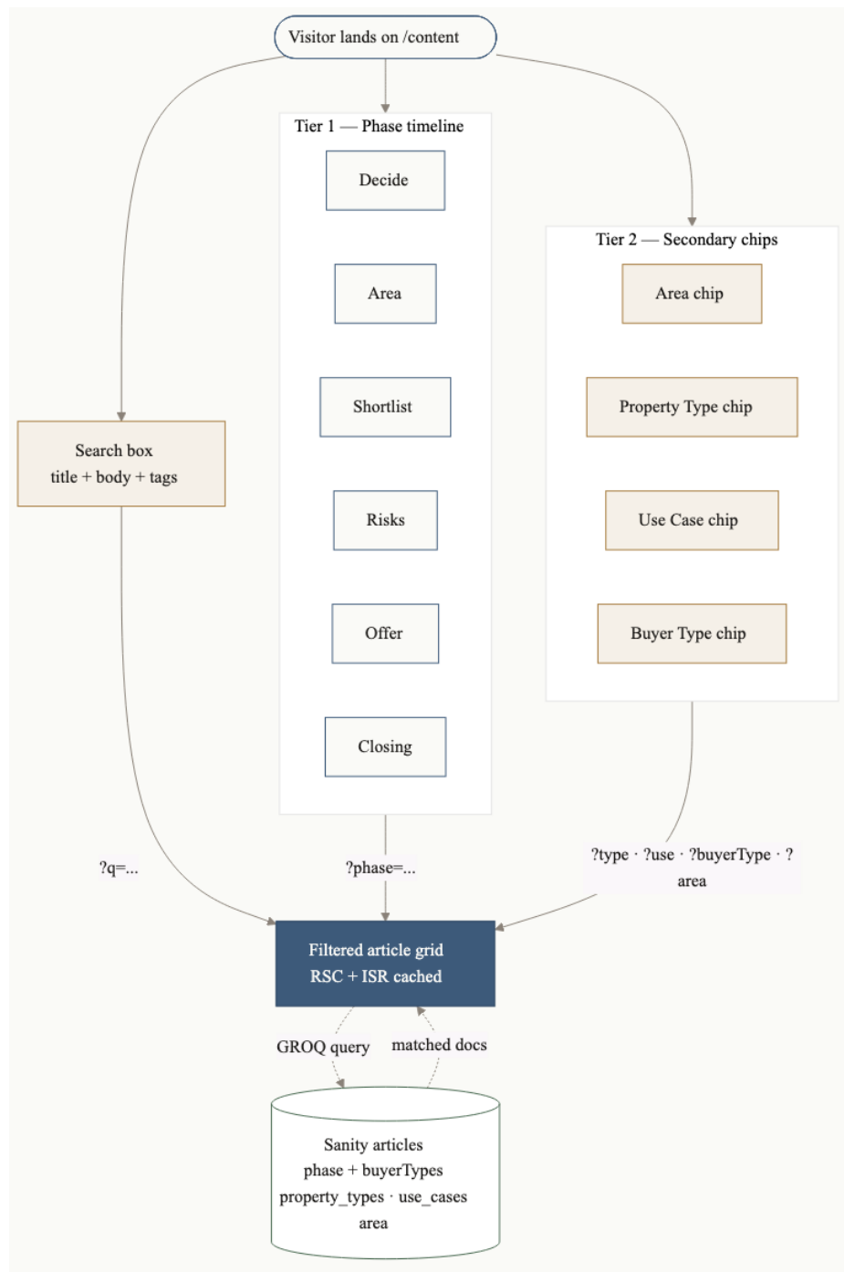
Content Hub filter
