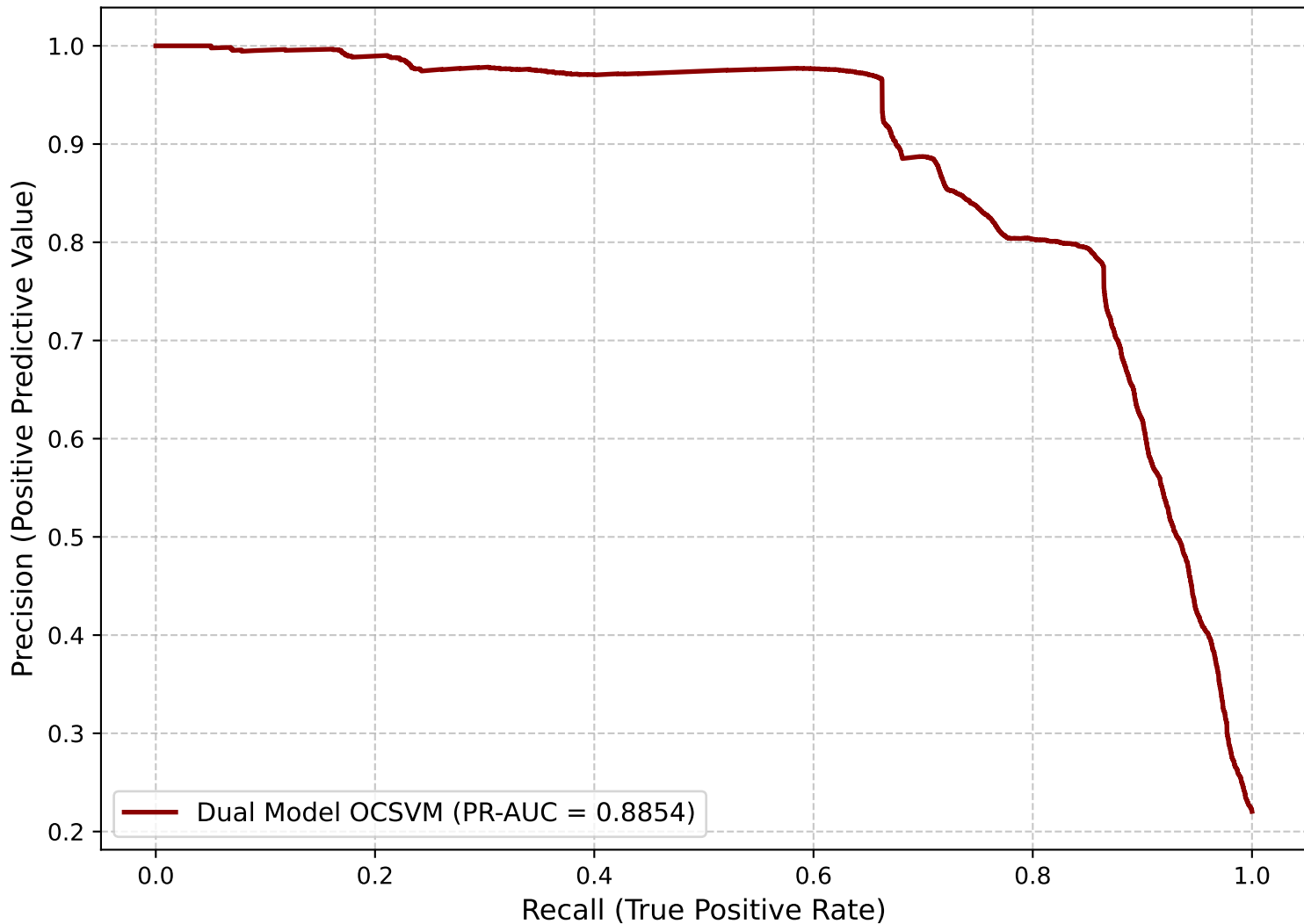
Precision-Recall Curve: Dual Model OCSVM
