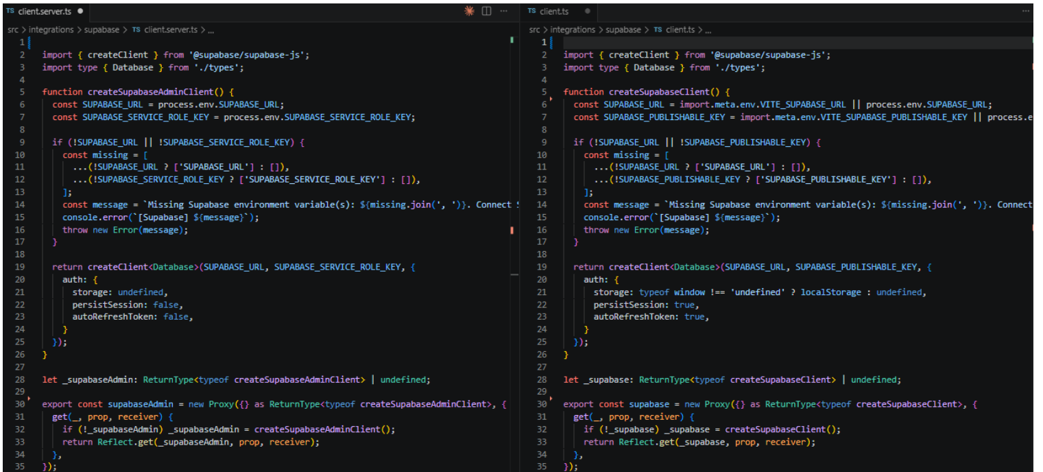
Figure 10. The Supabase client split: service-role client (left), browser client (right).
