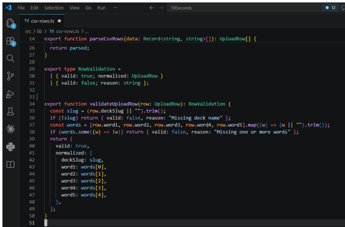
Figure 13. Row validation in src/lib/csv-rows.ts .
