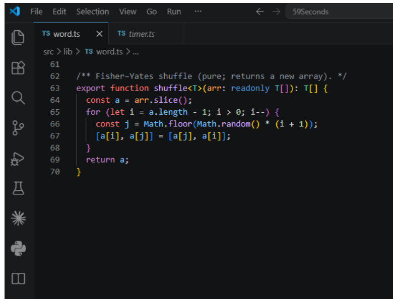
Figure 12. The Fisher-Yates shuffle in src/lib/word.ts .
