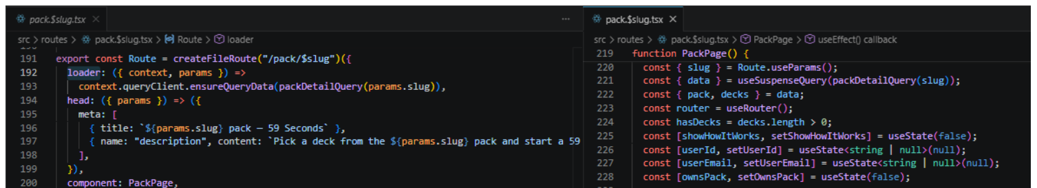
Figure 11. UI-to-backend linkage: the route loader prefetches the query the component consumes.
