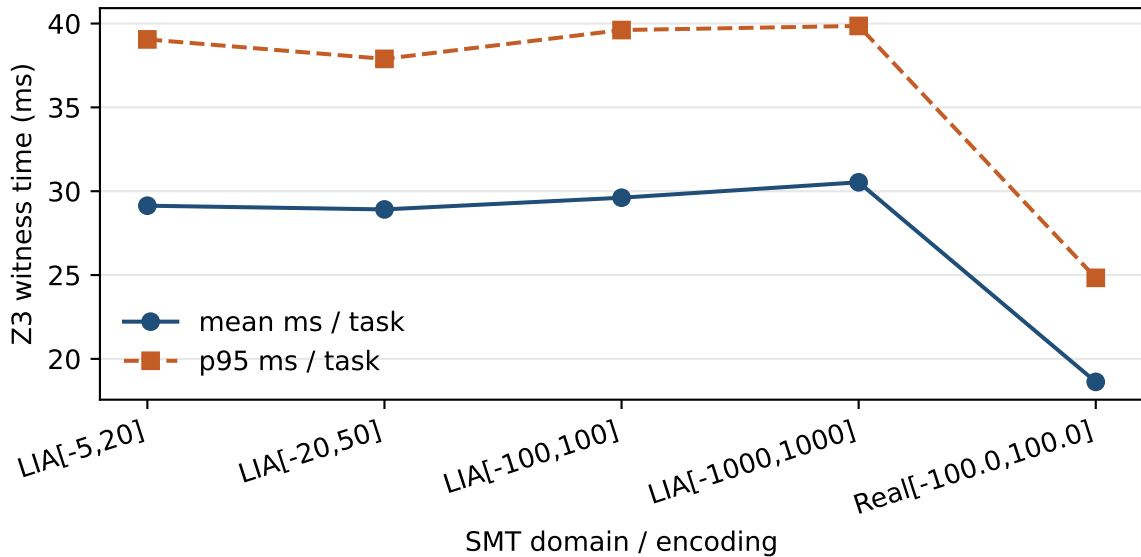
SMT scalability on real_priority_micro ( n = 30 )
