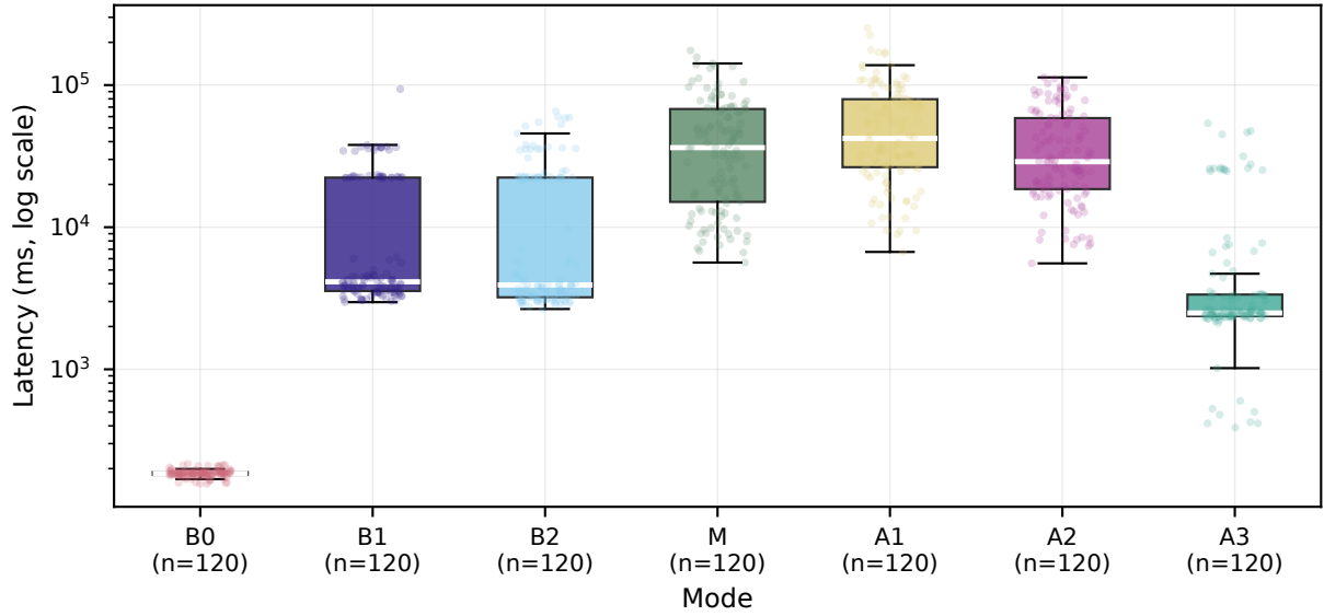
Fig. D.1. Archive figure (pre-fix E1 export): historical latency mass under the buggy others-witness oracle / hard gate. Authoritative cost story is fixed-oracle E1 (run_e1_m_win_v2): M 10.5s vs. B2 9.6s at comparable mean llm_calls ( \approx 1.16 vs. \approx 1.18 )—do not cite this figure as the current premium. How to read: log-scale wall-clock latency per task on the historical export only.
