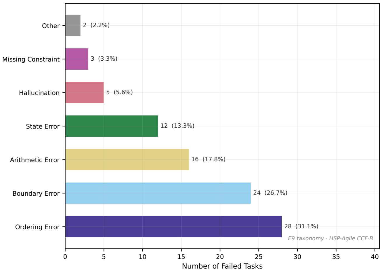
Residual error distribution — mode M ( n = 90 failed tasks)
