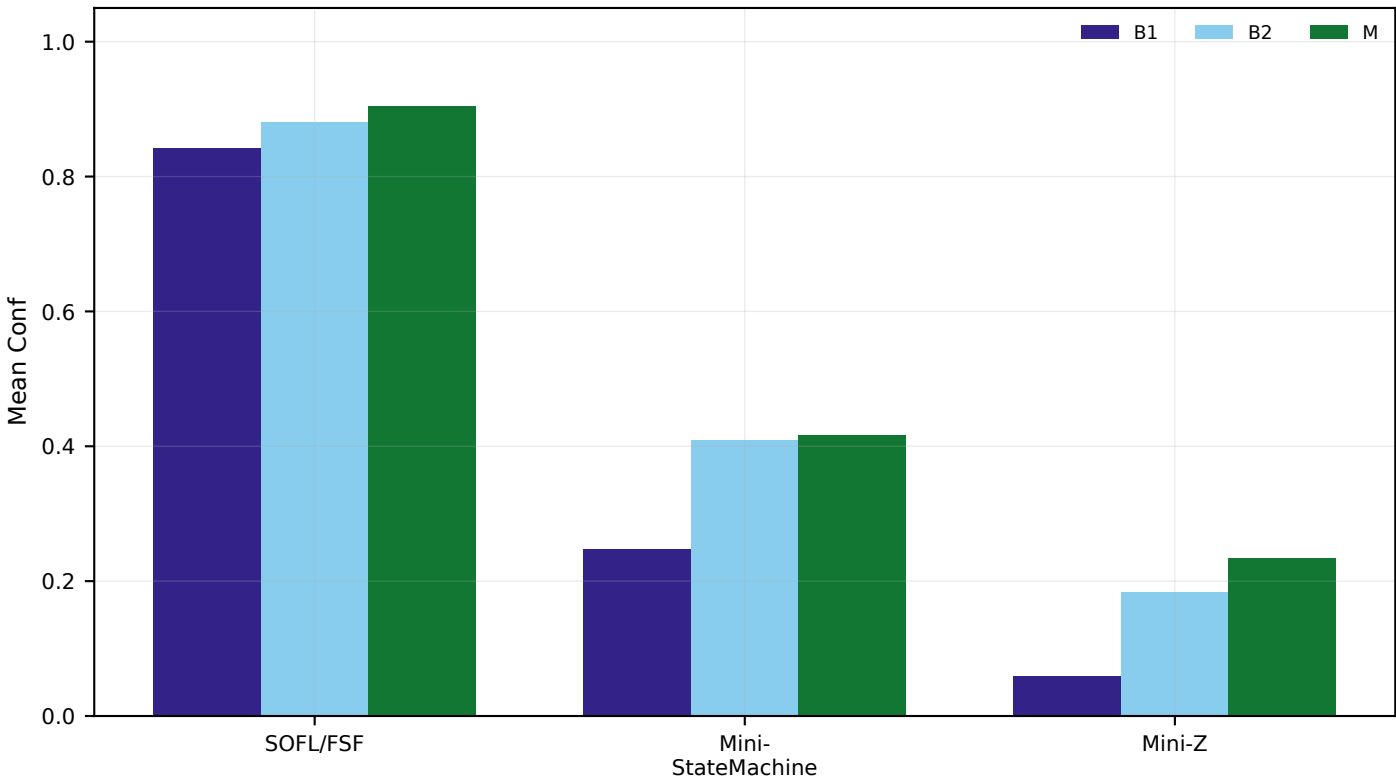
Generalisation across spec notations (E8)
