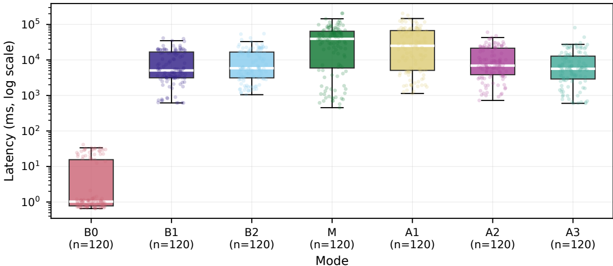
Latency Distribution by Mode (log scale)
