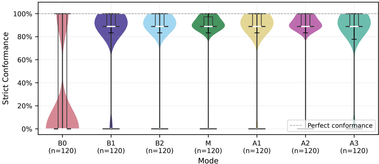
Strict Conformance Distribution by Mode
