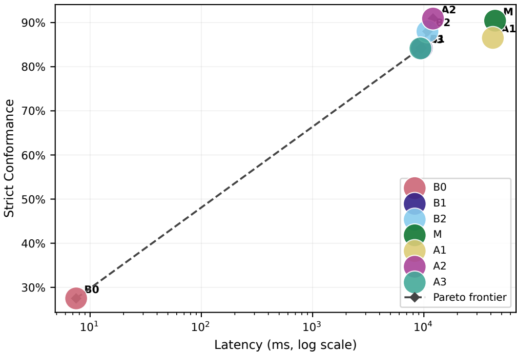
Pareto: Quality vs Latency
