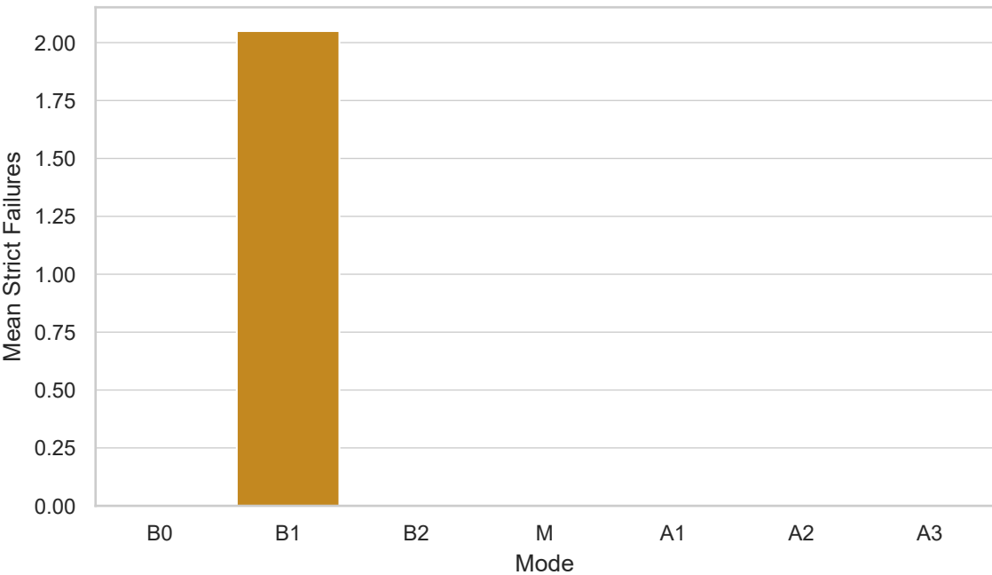
Strict Failure Burden by Mode
