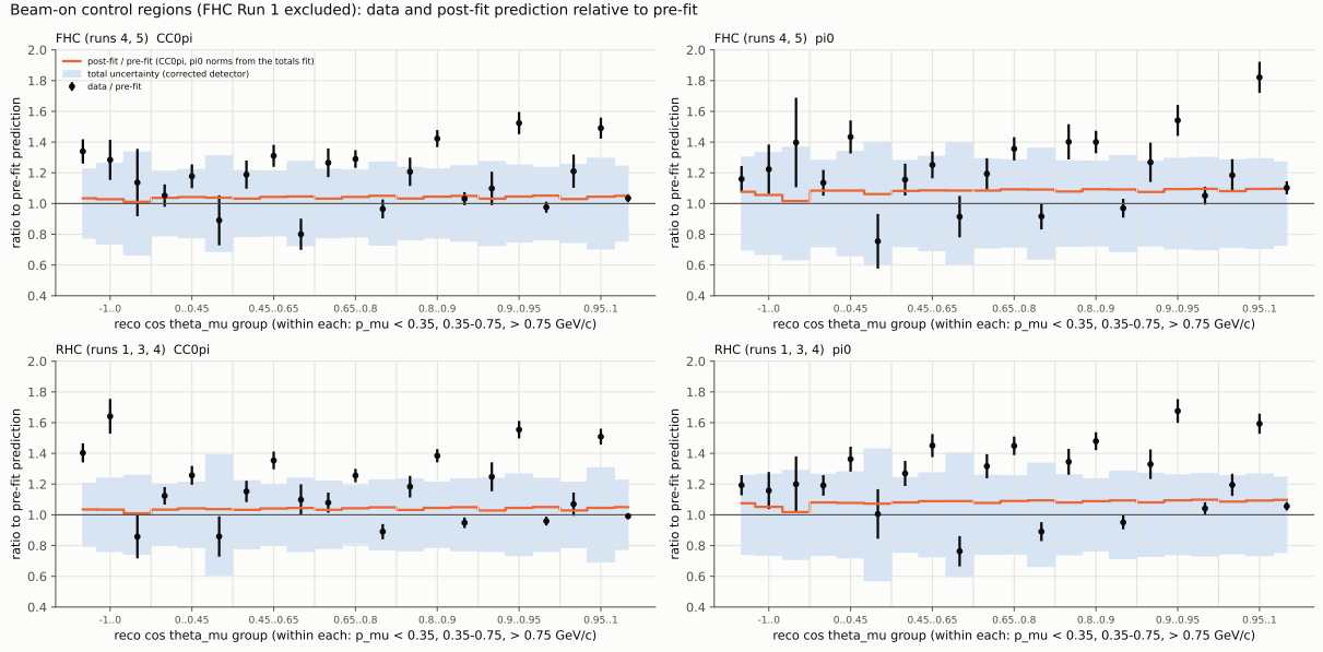
Figure 5: Beam-on control regions without FHC Run 1: data and the post-fit prediction (CC0 \pi and \pi^0 normalisations from the totals fit) relative to the pre-fit prediction, in reconstructed \cos\theta_\mu groups, each split into p_\mu < 0.35 , 0.35\text{--}0.75 , and > 0.75 GeV/c; band: total uncertainty.
