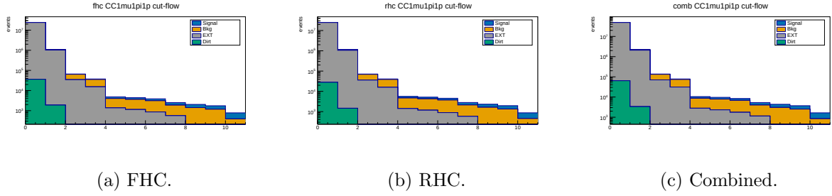
Figure 24: Proton-tagged ( \text{CC1}\mu 1\pi 1p ) cut-flow yields at full exposure (log scale; MC-prediction stack, Okabe-Ito: signal blue, background orange, EXT grey, dirt green). The last stage, IdentProton, is the leading-proton identification that defines the subsample.
