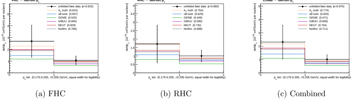
Figure 22: The two-bin p_\pi cross section, the graphical form of Tab. 14. Unfolded fake data (points, with the full systematic uncertainty) against the A_C -smeared truth, the uB tune and the four generators; every curve is A_C -smeared, so all of them live in the same space as the measurement. The two bins are drawn with equal width for legibility: they are 0.030 and 0.795 GeV/c wide, so to scale the first would occupy 4% of the axis. Area on these panels is therefore not proportional to cross section, and the integrated \sigma is printed on each panel instead. The generators bracket the data in every bin of every configuration, with NEUT closest and GENIE lowest throughout.
