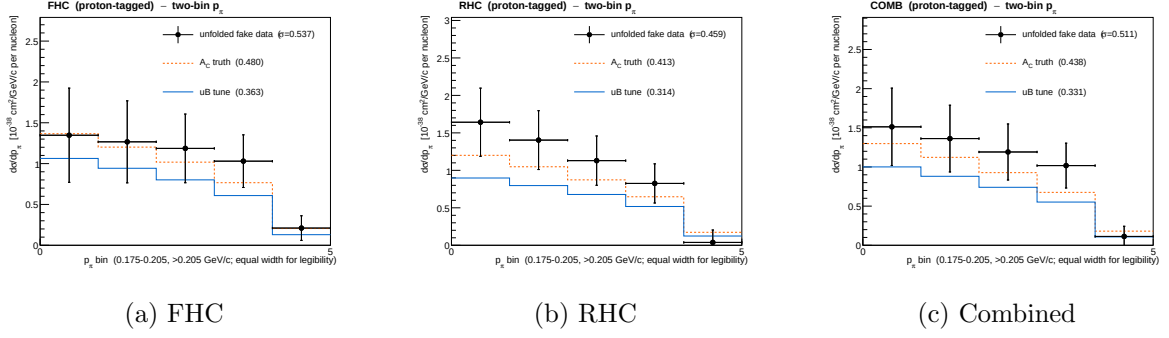
Figure 24: The two-bin p_\pi cross section on the proton-tagged CC1mu1pi1p selection, the graphical form of Tab. 16. Same edges as the inclusive result of Fig. 22 so the two are directly comparable, and the bins are again drawn equal-width.
