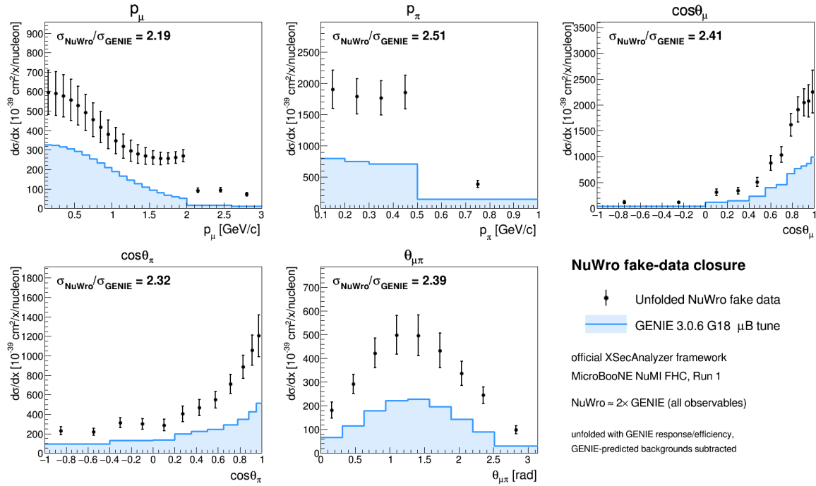
Figure 32: NuWro fake-data closure in the official XSECANALYZER framework. Points: unfolded NuWro fake data; shaded line: GENIE 3.0.6 G18 \mu\text{B} tune. The unfolded NuWro result sits a uniform \approx 2\times above the GENIE prediction in all five observables.
