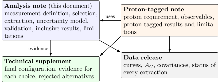
Figure 2: The documents of the analysis. The proton-tagged note takes the beam, exposure, samples, base selection, extraction and uncertainty model from this note; both notes refer to the technical supplement for the evidence behind their choices; the data release holds the numerical results of both.
