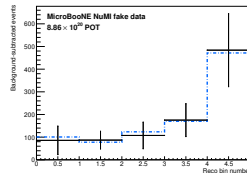
\cos \theta_\mu
