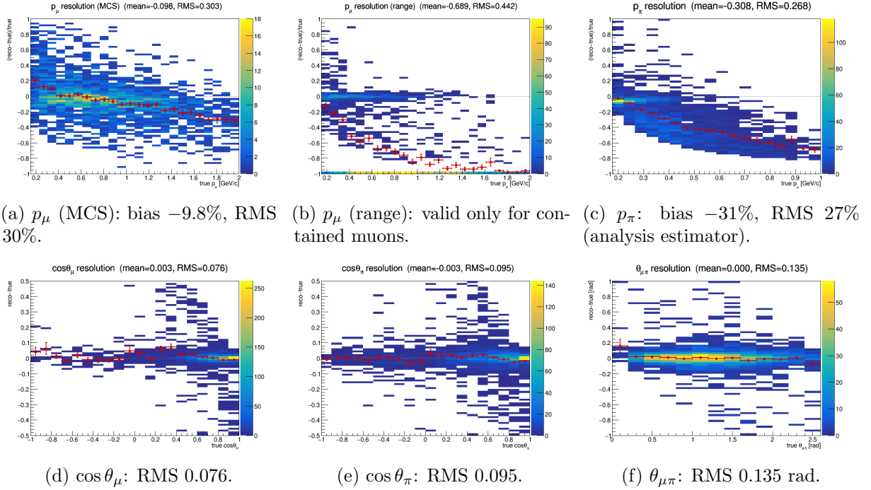
Figure 19: Reconstruction resolution vs. true value, selected signal. Momenta: relative (\text{reco} - \text{true})/\text{true} ; angles: absolute (\text{reco} - \text{true}) . Red points: mean residual per true bin. The muon MCS momentum slightly over-estimates at low p_\mu and increasingly under-estimates above \sim 1 GeV/ c ; the range estimator is badly biased for exiting muons (range = distance to wall), which is why the analysis uses range only for contained muons (range-or-MCS). The pion panel shows the estimator the analysis actually bins on, not the raw candidate_pion_mom_reco branch (§8.8): mean bias -31\% , RMS 27\% . That average is dominated by high momenta — the bias is only -2\% in the first true bin and reaches -65\% above 0.8 GeV/ c — because the reconstructed value saturates near 0.34 GeV/ c once pions interact hadronically before stopping. The angular variables are essentially unbiased with narrow resolution.
