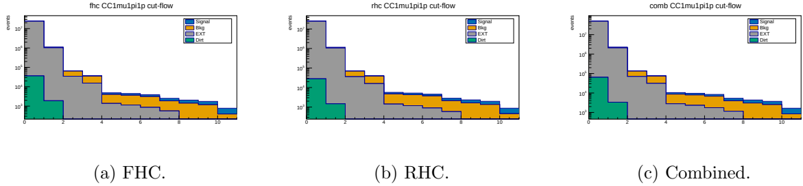
Figure 24: Proton-tagged ( CC1mu1pi1p ) cut-flow yields at full exposure (log scale; MC-prediction stack, Okabe-Ito: signal blue, background orange, EXT grey, dirt green). The last stage, IdentProton, is the leading-proton identification that defines the subsample.
