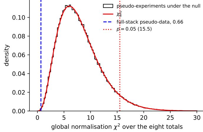
Figure 10: Null calibration of the global normalisation \chi^2 over the eight (region, mode) totals: 2 \times 10^5 pseudo-experiments with the prediction drawn from its pre-fit covariance and Poisson-fluctuated data, against the \chi^2_8 density. The full-stack pseudo-data value 0.66 is marked; it is low because the pseudo-data is a Poisson throw of the same prediction and carries none of the prediction’s systematic variation.
