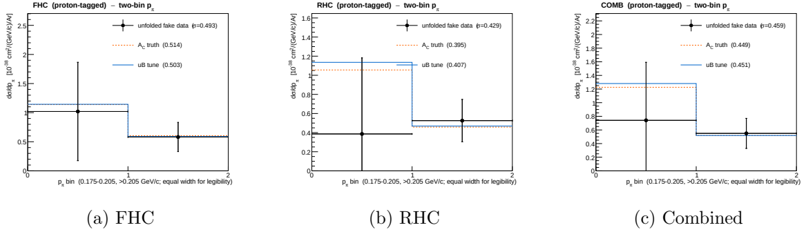
Figure 4: The two-bin p_\pi cross section on the proton-tagged CC1mu1pi1p selection, the graphical form of Tab. 4. The first bin is that of the inclusive result of Fig. 2, and the second is the union of the two upper inclusive regions, since three regions fail the 0.50 criterion in this sample. The bins are drawn equal-width.
