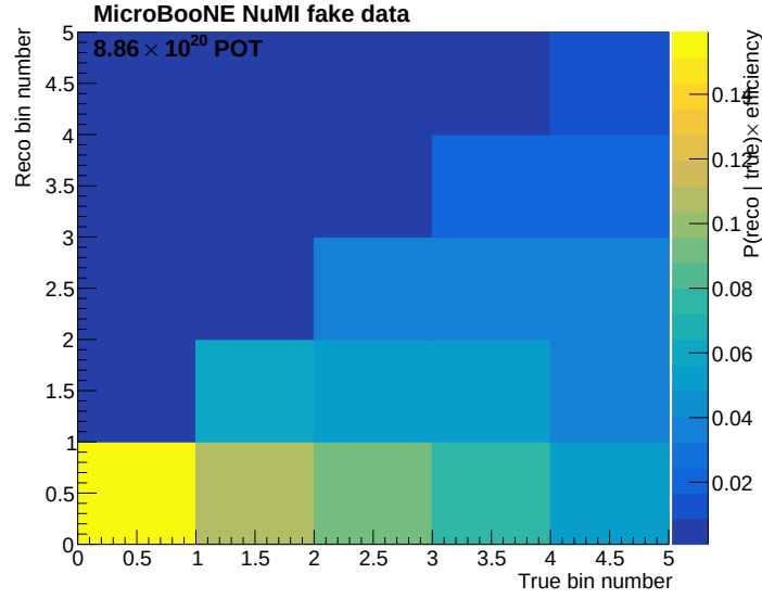
Figure 13: Smearceptance matrix of the rejected five-bin p_\pi scheme (FHC): reconstructed events pile into the lowest bin from every true bin, the diagnostic that motivated the merged regions of §2.1.6; the released three-region response is in the analysis note.
