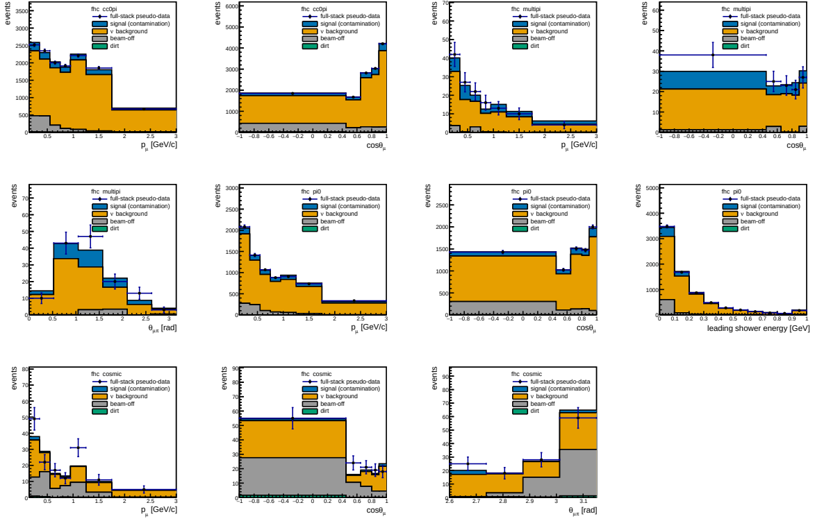
Figure 7: FHC control-region distributions at the frozen binning (the frozen plotting list): by row, CC0 \pi , multi- \pi , \pi^0 and cosmic; p_\mu , \cos \theta_\mu and, where defined, the muon-pion opening angle or the leading shower energy. Stack: signal contamination, neutrino background, beam-off (per-run scaled) and dirt; points: full-stack pseudo-data (neutrino-MC throw plus a Poisson throw of the beam-off and dirt expectations). These are the plots the collaboration will see with beam-on points after opening; overflow is in the last bin.
