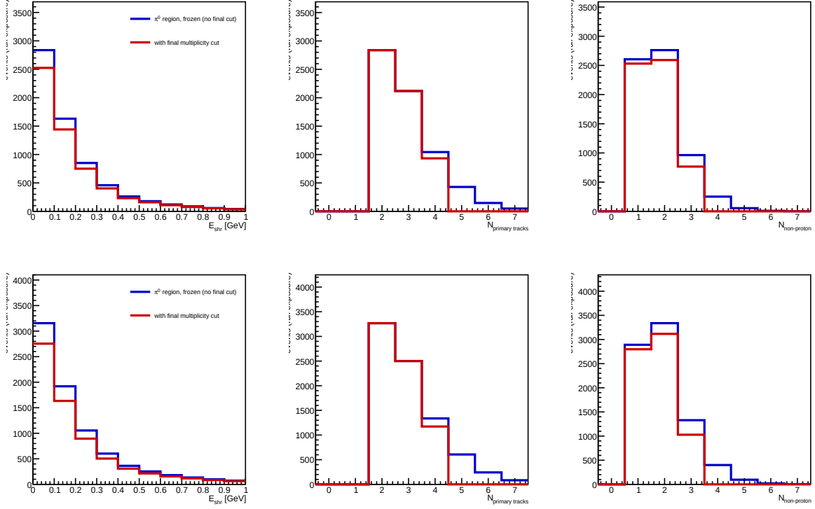
Figure 9: The \pi^0 region without (blue) and with (red) the final multiplicity cut, FHC (top) and RHC (bottom), neutrino MC at full exposure: the leading shower energy, the number of primary tracks and the number of non-proton-like tracks.
