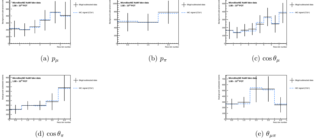
Figure 12: Stage 2, combined: background-subtracted data compared with the central-value MC signal.
