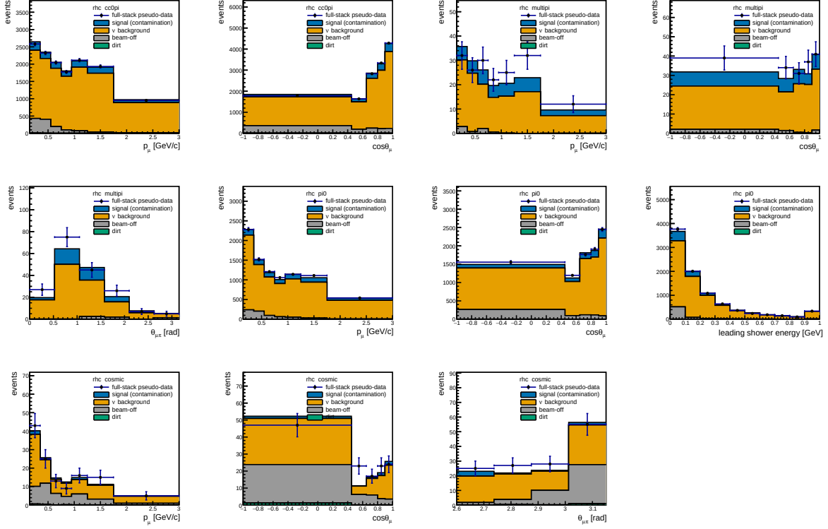
Figure 8: As Fig. 7, for RHC.
