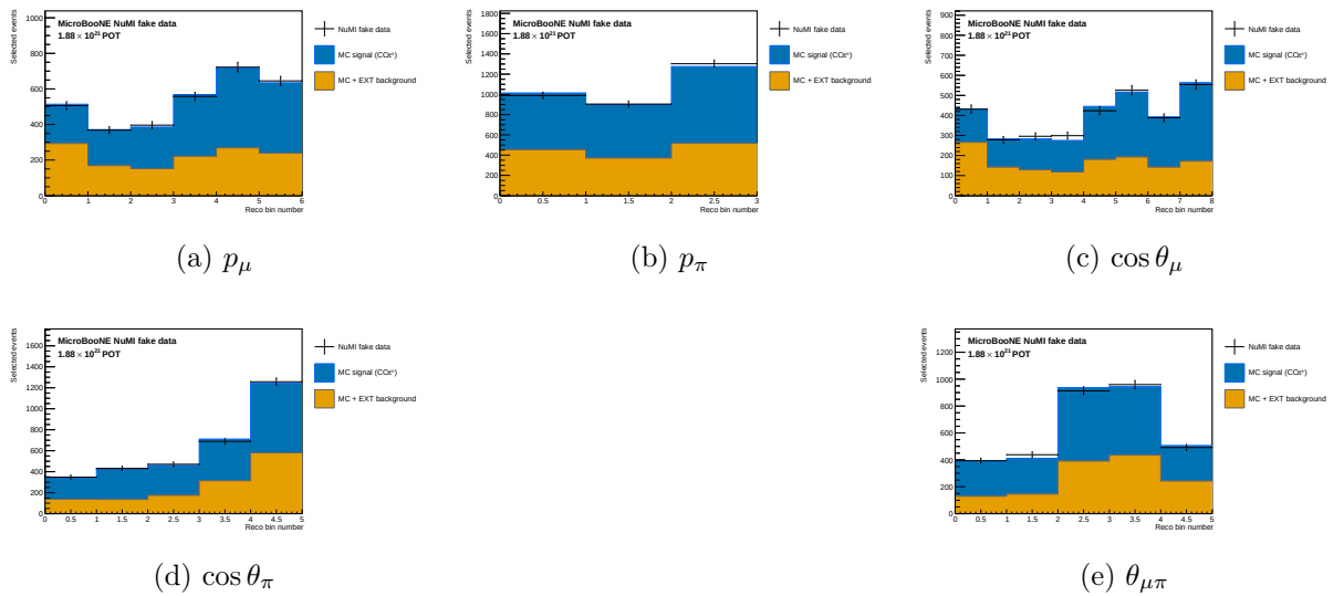
Figure 11: Stage 1, combined: selected reconstructed spectra at the combined FHC+RHC exposure.
