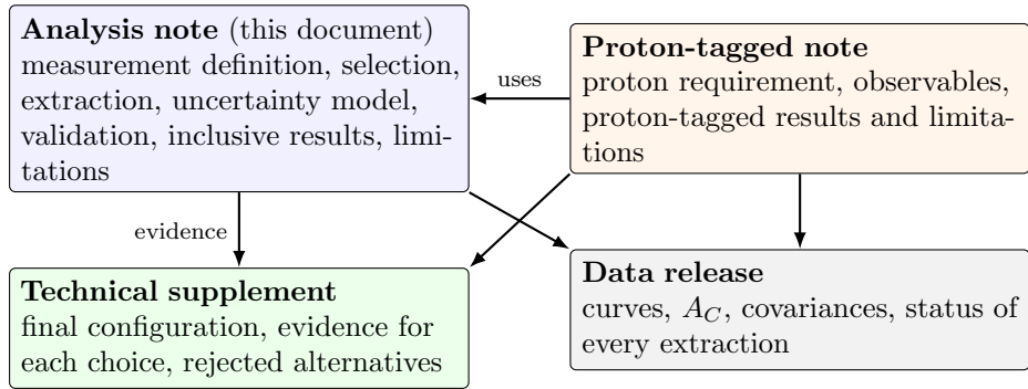
Figure 2: The documents of the analysis. The proton-tagged note takes the beam, exposure, samples, base selection, extraction and uncertainty model from this note; both notes refer to the technical supplement for the evidence behind their choices; the data release holds the numerical results of both.
