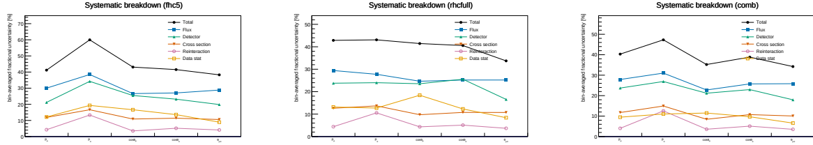
Figure 23: Bin-averaged fractional systematic uncertainty by source vs. observable, for FHC (left), RHC (centre) and combined (right); the figure form of Table 22 of the technical supplement–Table 24 of the technical supplement. Colours use the Okabe-Ito colourblind-safe palette with distinct markers per source: total (black), flux (blue), detector (green), cross section (vermillion), reinteraction (purple), data stat (orange).
