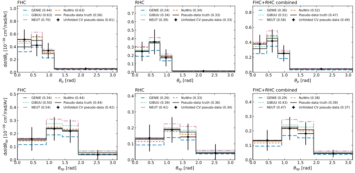
Figure 1: The two proton angles in the three configurations: \theta_p (top row) and \theta_{np} (bottom row), for FHC, RHC and combined. Points are the unfolded pseudo-data with the total uncertainty, the grey histogram is the A_C -smeared pseudo-data truth, and the four coloured histograms are the generator predictions; the integrated cross sections are given in the legends.
