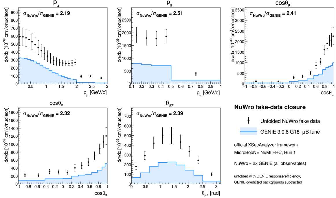
Figure 7: [HISTORICAL — 2026-07-25, not regenerated.] This figure predates the central-value weighting fix, the width-aware regularisation and the removal of the duplicated A_C , and it has no producer in the repository, so it cannot be rebuilt from the current state. What survives it is the qualitative point — a NuWro-over- GENIE ratio of order two, which is a genuine generator difference — not the absolute normalisation or the model curve, the latter of which carries the double smearing. NuWro fake-data closure in the official XSECANALYZER framework. Points: unfolded NuWro fake data; shaded line: GENIE 3.0.6 G18 \mu B tune. The unfolded NuWro result sits a uniform \approx 2\times above the GENIE prediction in all five observables. This figure predates the fake-data weighting fix of Sec. 16 of the analysis note: it was produced 2026-07-25, from a separate cross-pipeline study, and has no producer in the repository. The \approx 2\times NuWro-over-GENIE ratio it shows is a generator comparison and survives the fix; the absolute normalisation of the points does not. Retained as a qualitative cross-pipeline check only.
