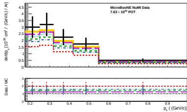
(a) d\sigma/dp_\pi (framework, optimised binning).
