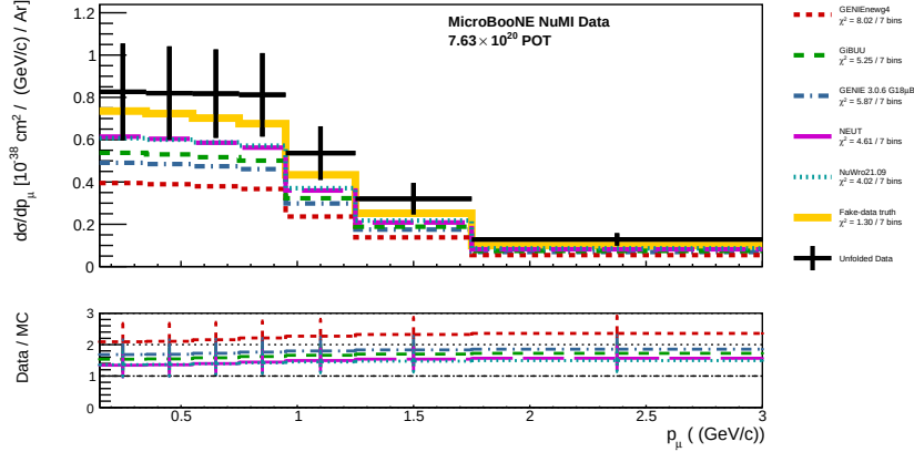
Figure 37: Unfolded d\sigma/dp_\mu (fake data) on the optimised binning (§3.8): four generators (GENIE, GiBUU, NuWro, NEUT) + MicroBooNE tune + fake-data truth (all A_C -smeared), with data/MC ratio panel.
