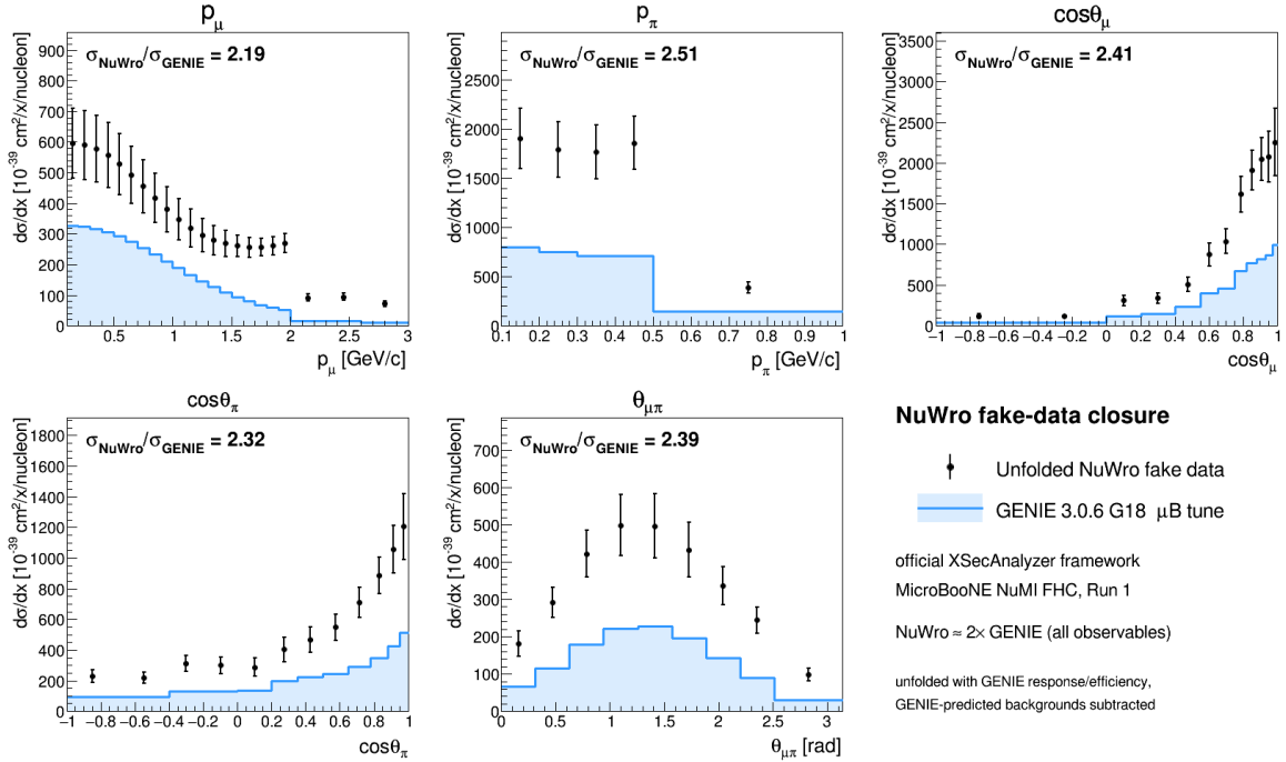
Figure 20: NuWro fake-data closure in the official XSECANALYZER framework. Points: unfolded NuWro fake data; shaded line: GENIE 3.0.6 G18 \mu\text{B} tune. The unfolded NuWro result sits a uniform \approx 2\times above the GENIE prediction in all five observables.
