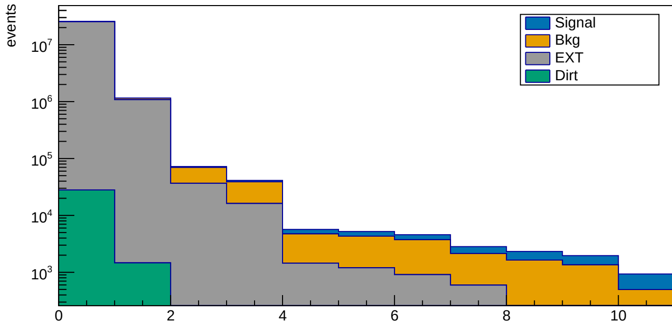
rhc CC1mu1pi1p cut-flow
