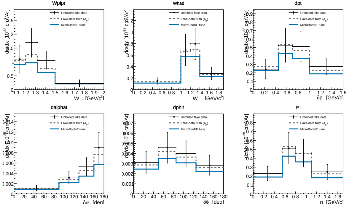
Figure 17: Proton-tagged (CC1mu1pi1p) differential cross sections for FHC: the \pi p invariant mass W_{\pi p} , the calorimetric hadronic mass W_{\text{had}} , and the four transverse-kinematic-imbalance observables \delta p_T , \delta\alpha_T , \delta\phi_T and p_n . Unfolded fake data (black points) are compared to the A_C -smeared fake-data truth (grey dashed) and the MicroBooNE tune (blue). W_{\pi p} falls from the \Delta(1232) threshold region; \delta\alpha_T rises toward 180^\circ , the signature of final-state interactions.
