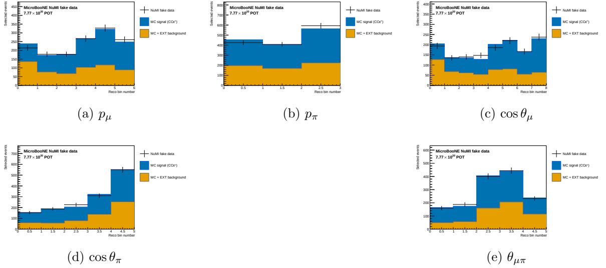
Figure 12: Stage 1, FHC: selected reconstructed spectra scaled to the full exposure, with the MC split into signal and background. Points are the Poisson-thrown pseudo-data. The RHC equivalent is Fig. 14 and the combined one Fig. 9 of the technical supplement.
