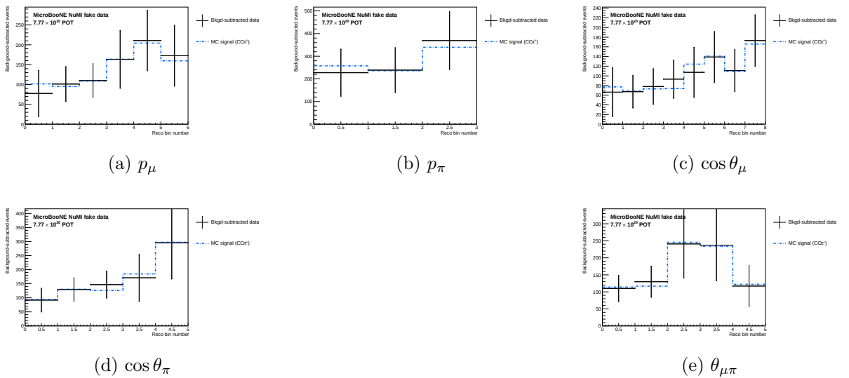
Figure 13: Stage 2, FHC: background-subtracted data compared with the central-value MC signal; the input to the unfolding. RHC: Fig. 15; combined: Fig. 10 of the technical supplement.
