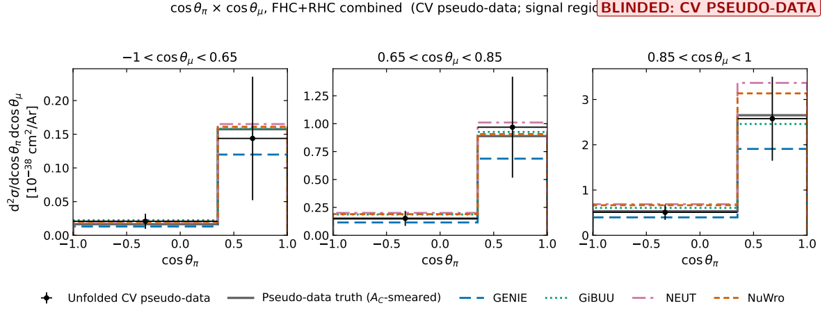
Figure 26: d^2\sigma/d\cos\theta_\pi d\cos\theta_\mu in the combined configuration, as slices in \cos\theta_\mu . Points are the unfolded pseudo-data with the total uncertainty, the grey histogram is the A_C -smeared truth of the pseudo-data and the coloured histograms are the generator predictions, smeared with A_C . Each slice has its own vertical scale.
