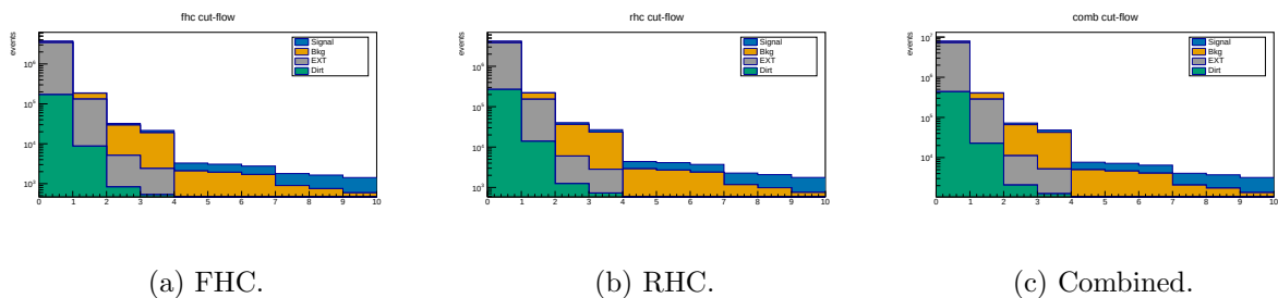
Figure 4: Cut-flow yields at full exposure for FHC, RHC and combined (log scale; MC-prediction stack: signal blue, background orange, EXT grey, dirt green), with signal and background scaled per run to the recorded exposure. The detailed breakdown by category is in Table 11.
