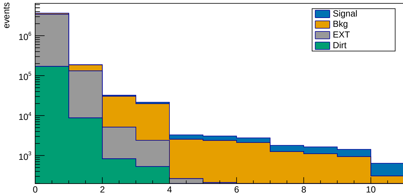
fhc CC1mu1pi1p cut-flow
