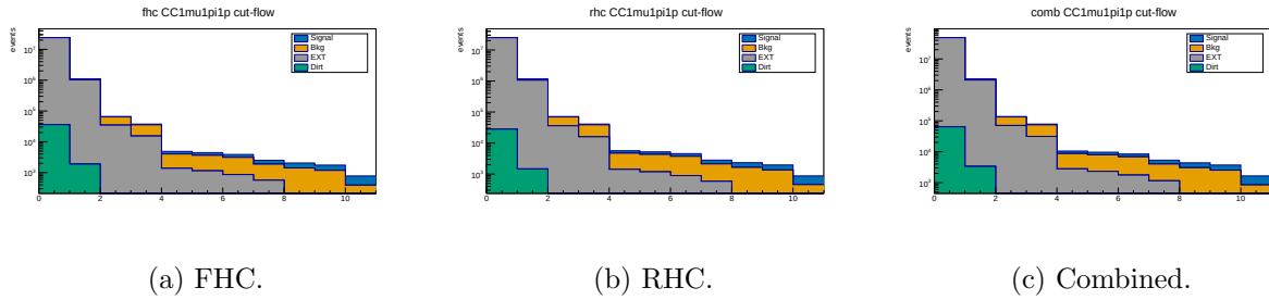
Figure 29: Proton-tagged ( CC1mu1pi1p ) cut-flow yields at full exposure (log scale; MC-prediction stack, Okabe-Ito: signal blue, background orange, EXT grey, dirt green). The last stage, IdentProton, is the leading-proton identification that defines the subsample.
