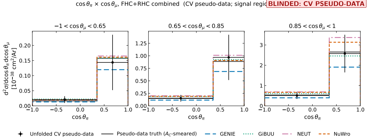
Figure 26: d^2\sigma/d\cos\theta_\pi d\cos\theta_\mu in the combined configuration, as slices in \cos\theta_\mu . Points are the unfolded pseudo-data with the total uncertainty, the grey histogram is the A_C -smeared truth of the pseudo-data and the coloured histograms are the generator predictions, smeared with A_C . Each slice has its own vertical scale.
