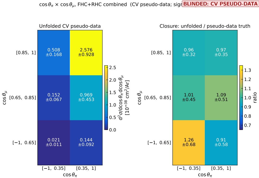
Figure 27: The same result as a map: d^2\sigma/d\cos\theta_\pi d\cos\theta_\mu per cell with its total uncertainty (left) and the ratio to the A_C -smeared truth (right). Cells are drawn with equal size and labelled by their ranges.
