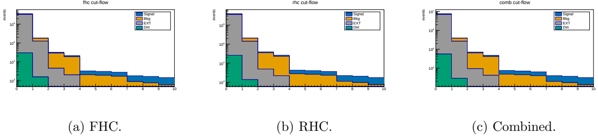
Figure 5: Cut-flow yields at full exposure for FHC, RHC and combined (log scale; MC-prediction stack: signal blue, background orange, EXT grey, dirt green; colourblind-safe Okabe-Ito palette), with signal and background scaled per run to the recorded exposure. The detailed breakdown by category is in Table 12.
