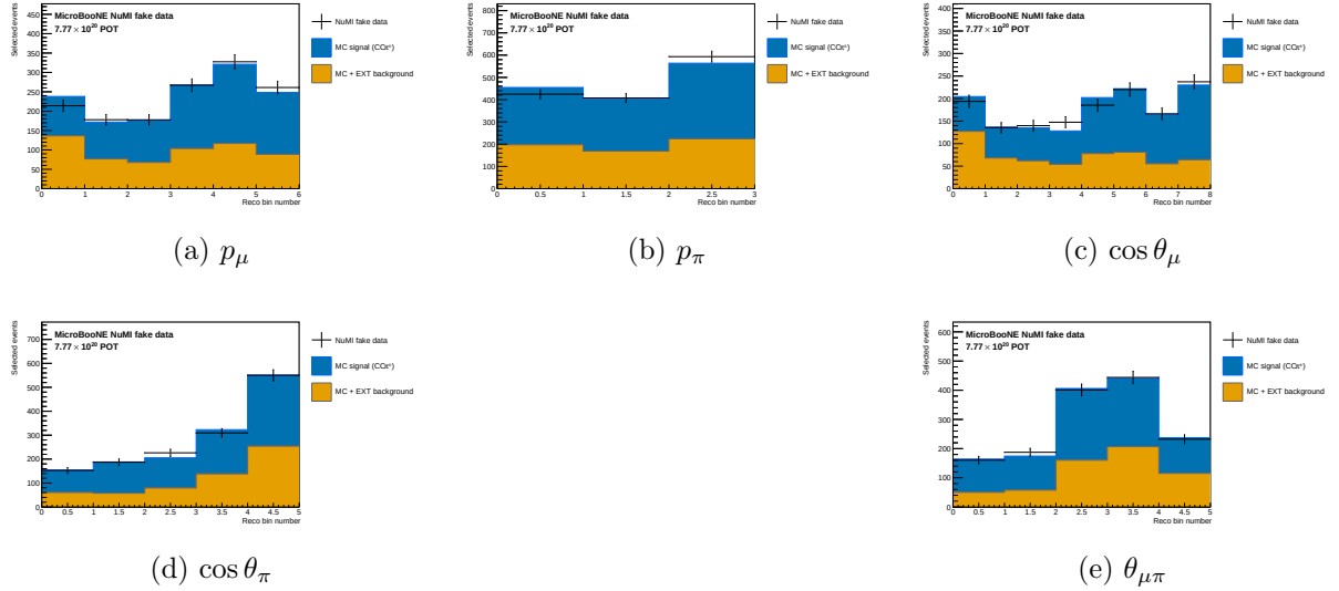
Figure 13: Stage 1, FHC: selected reconstructed spectra scaled to the full exposure, with the MC split into signal and background. Points are the Poisson-thrown pseudo-data. The RHC equivalent is Fig. 15 and the combined one Fig. 13 of the technical supplement.
