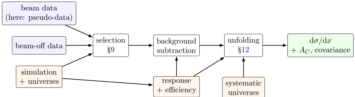
Figure 2: The extraction chain. The same selection is applied to data, beam-off data and simulation; the simulation also supplies the response and the systematic universes. The output is a cross section together with the additional-smearing matrix A_C and the covariance, all three of which are needed to compare the result with a prediction.
