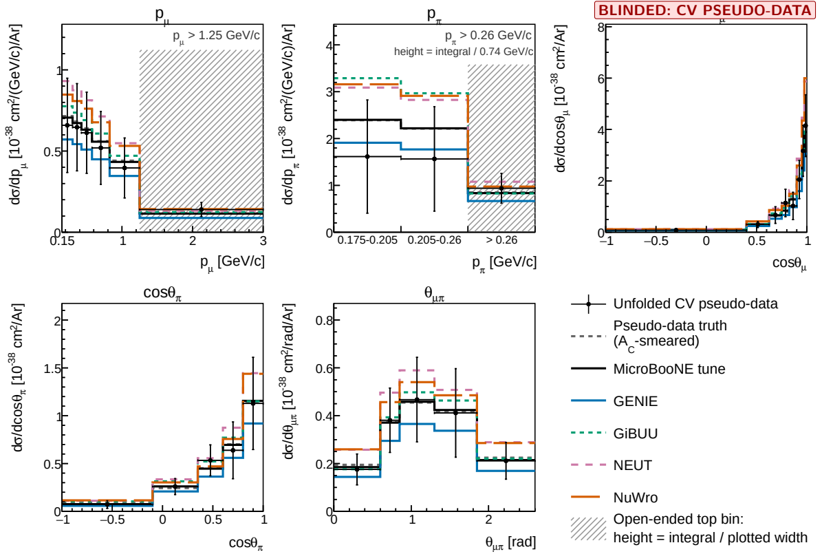
Figure 24: Differential cross sections d\sigma/dx of the five distributions, FHC full exposure, extracted from pseudo-data. The points are the Wiener-SVD estimator A_C x_{\text{true}} ; shown are the unfolded pseudo-data (black points), the A_C -smeared truth of the pseudo-data (grey dashed), the MicroBooNE tune (black solid) and the four generator predictions (GENIE, GiBUU, NEUT, NuWro), all smeared with A_C . The unfolded points recover the injected truth in every observable, the closure summarised in Table 22.
