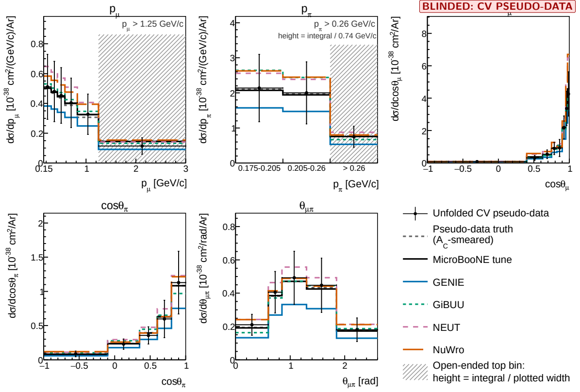
Figure 25: RHC differential cross sections from pseudo-data, with the generator predictions averaged over the RHC flux. Same layout as Fig. 24.
