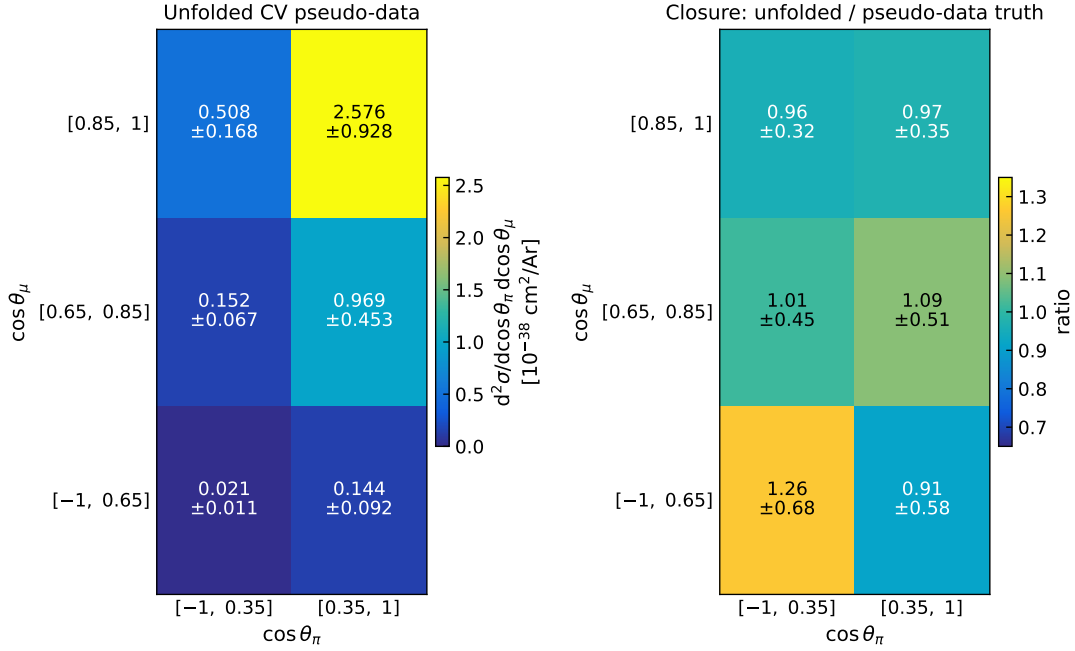
Figure 28: The same result as a map: d^2\sigma/d\cos\theta_\pi d\cos\theta_\mu per cell with its total uncertainty (left) and the ratio to the A_C -smeared truth (right). Cells are drawn with equal size and labelled by their ranges.
