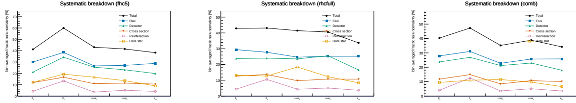
Figure 23: Bin-averaged fractional systematic uncertainty by source vs. observable, for FHC (left), RHC (centre) and combined (right); the figure form of Table 24 of the technical supplement–Table 26 of the technical supplement. Colours use the Okabe-Ito colourblind-safe palette with distinct markers per source: total (black), flux (blue), detector (green), cross section (vermillion), reinteraction (purple), data stat (orange).
