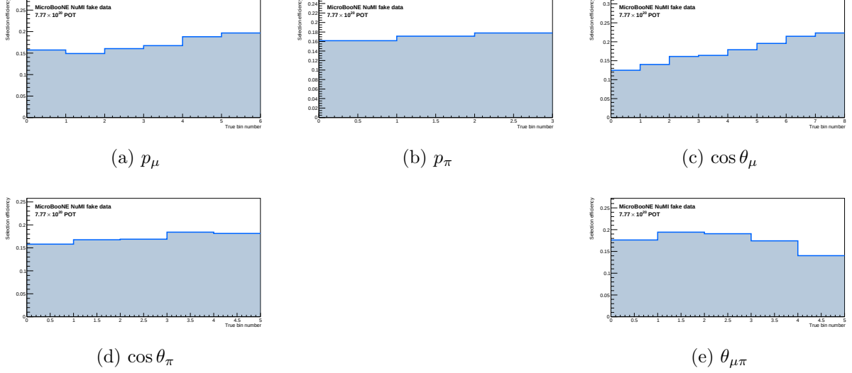
Figure 21: Selection efficiency as a function of true observable value, in the measured phase space ( p_\mu > 0.15 , p_\pi > 0.175 GeV/c, \theta_{\mu\pi} < 2.6 rad). Efficiency is the ratio of selected to generated signal MC ( \varepsilon_j = \sum_i S_{ij} , summed over reconstructed bins). With the momentum thresholds and the 2.6 rad opening-angle cut the efficiency is flat at 13–20% across all observables; the low-momentum turn-on and the large-angle region dominated by cosmic rays lie outside the measured phase space. The lowest point is the smallest opening-angle bin (9% efficiency), which is kept because its purity is high (58%).
