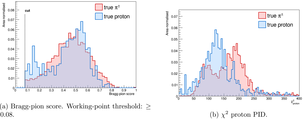
Figure 7: Pion-candidate PID distributions for true \pi^\pm (red) and true protons (blue) at the final cut stage. The Bragg-pion score provides the proton rejection; \chi_p^2 is shown as a cross-check.
