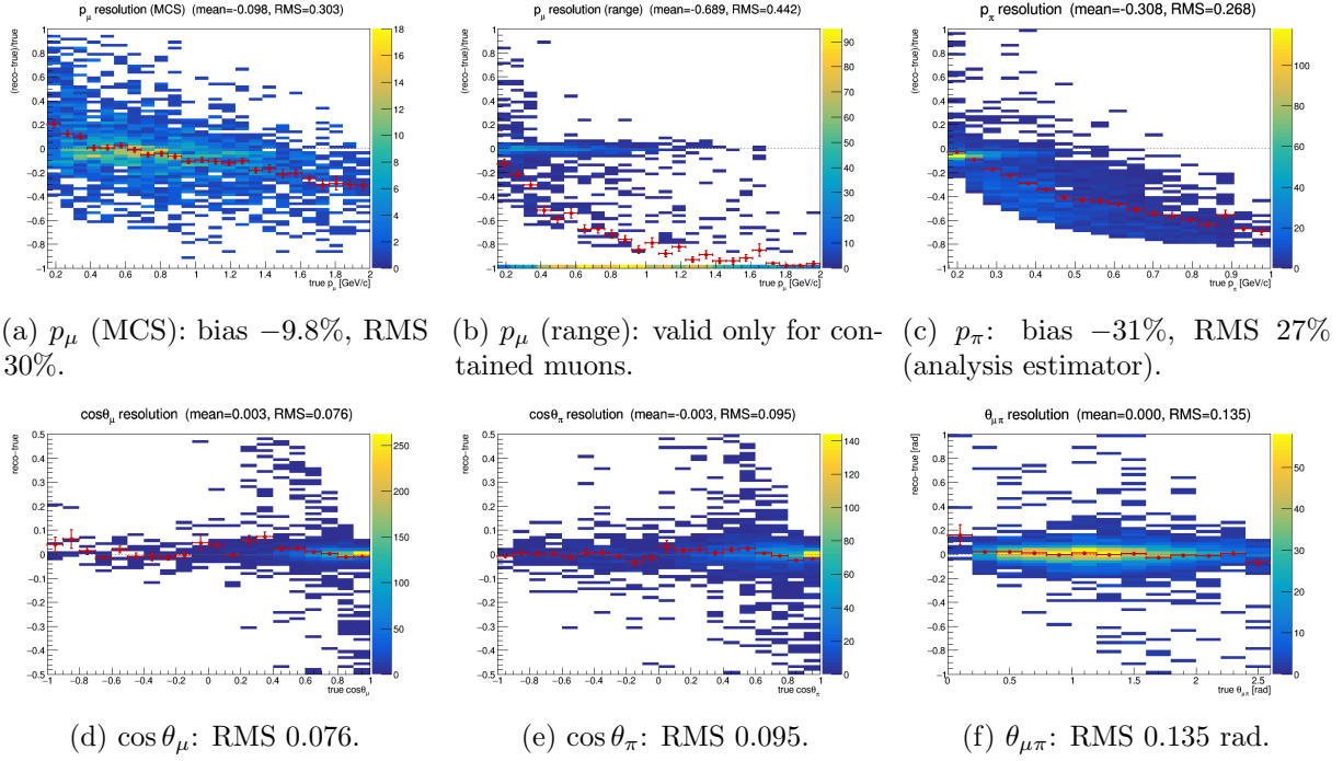
Figure 22: Reconstruction resolution vs. true value, selected signal. Momenta: relative ( \text{reco} - \text{true} )/ \text{true} ; angles: absolute ( \text{reco} - \text{true} ). Red points: mean residual per true bin. The muon MCS momentum slightly over-estimates at low p_\mu and increasingly under-estimates above \sim 1 GeV/ c ; the range estimator is badly biased for exiting muons (range = distance to wall), which is why the analysis uses range only for contained muons (range-or-MCS). The pion panel shows the estimator the analysis actually bins on, not the raw muon-hypothesis range momentum (Sec. 7.2 of the technical supplement): signed mean bias b = -31\% , RMS 27\% . That average is dominated by high momenta; b is only -2\% in the first true bin and reaches -65\% above 0.8 GeV/ c , because the reconstructed value saturates near 0.34 GeV/ c once pions interact hadronically before stopping. The angular variables are largely unbiased with narrow resolution.
