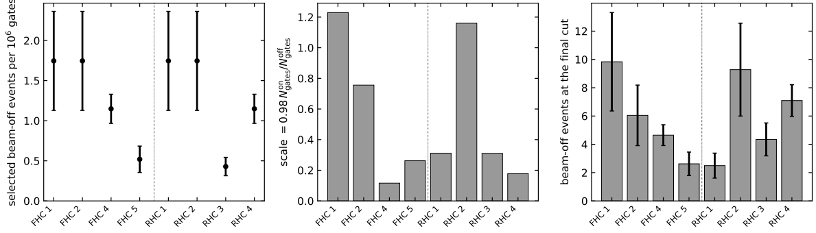
Figure 4: Beam-off normalisation by run period ( data_release/ext_gates.tsv ): selected beam-off rate per 10^6 gates at the final inclusive cut, with its Poisson uncertainty (left), the scale factor 0.98 \times (\text{beam-on gates}) / (\text{beam-off gates}) (centre), and the resulting beam-off events at the final cut (right), for each beam-on run period of the FHC and RHC configurations. Run 2 of both modes uses the Run-1 sample. The Run-1 rate is 1.5 to 4 times the rates of the later periods.
