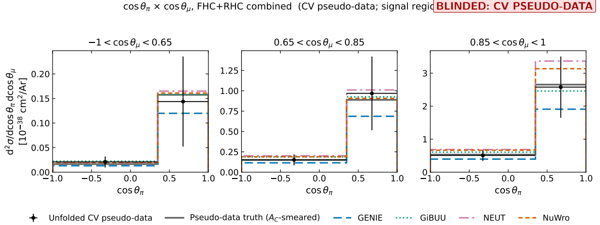
Figure 27: d^2\sigma/d\cos\theta_\pi d\cos\theta_\mu in the combined configuration, as slices in \cos\theta_\mu . Points are the unfolded pseudo-data with the total uncertainty, the grey histogram is the A_C -smeared truth of the pseudo-data and the coloured histograms are the generator predictions, smeared with A_C . Each slice has its own vertical scale.
