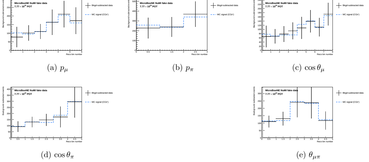
Figure 14: Stage 2, FHC: background-subtracted data compared with the central-value MC signal; the input to the unfolding. RHC: Fig. 16; combined: Fig. 14 of the technical supplement.
