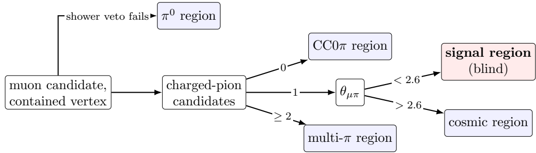
Figure 12: The four control regions and the signal region. Each region inverts one requirement of the signal selection, so no event belongs to a control region and to the signal region; this allows the control regions to be compared with beam-on data while the signal region remains blind.
