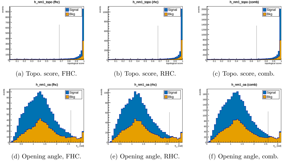
Figure 6: N–1 distributions for the topological score (Cut 3, top) and \mu – \pi opening angle (Cut 9, bottom), for FHC, RHC and combined. Signal (blue) and background (orange) stacked; dashed line = applied threshold. Colourblind-safe Okabe-Ito palette.
