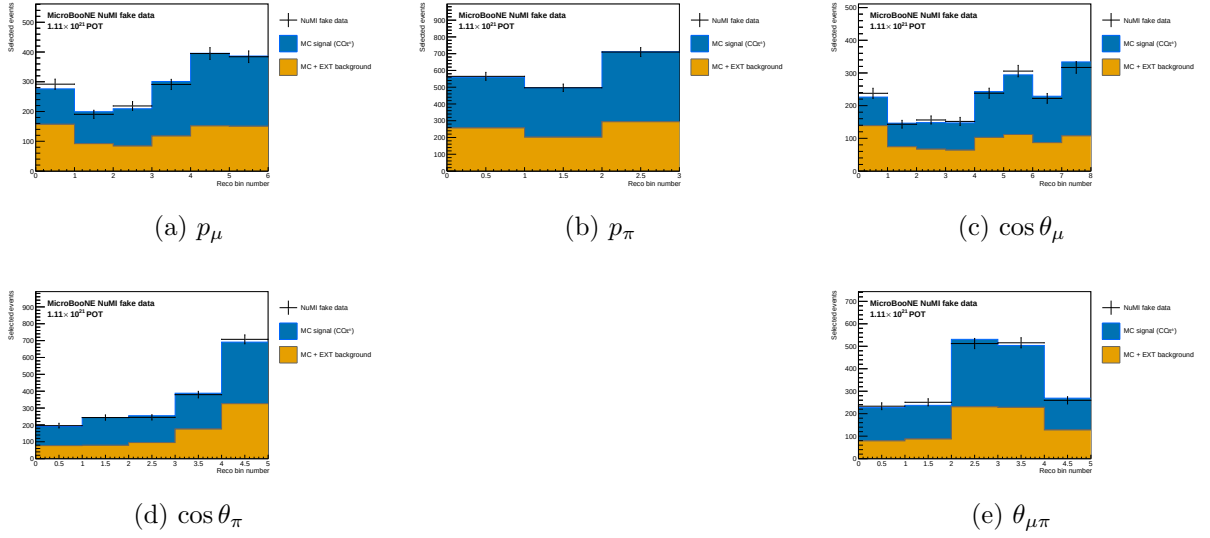
Figure 15: Stage 1, RHC: selected reconstructed spectra scaled to the full RHC exposure, MC split into signal and background.
