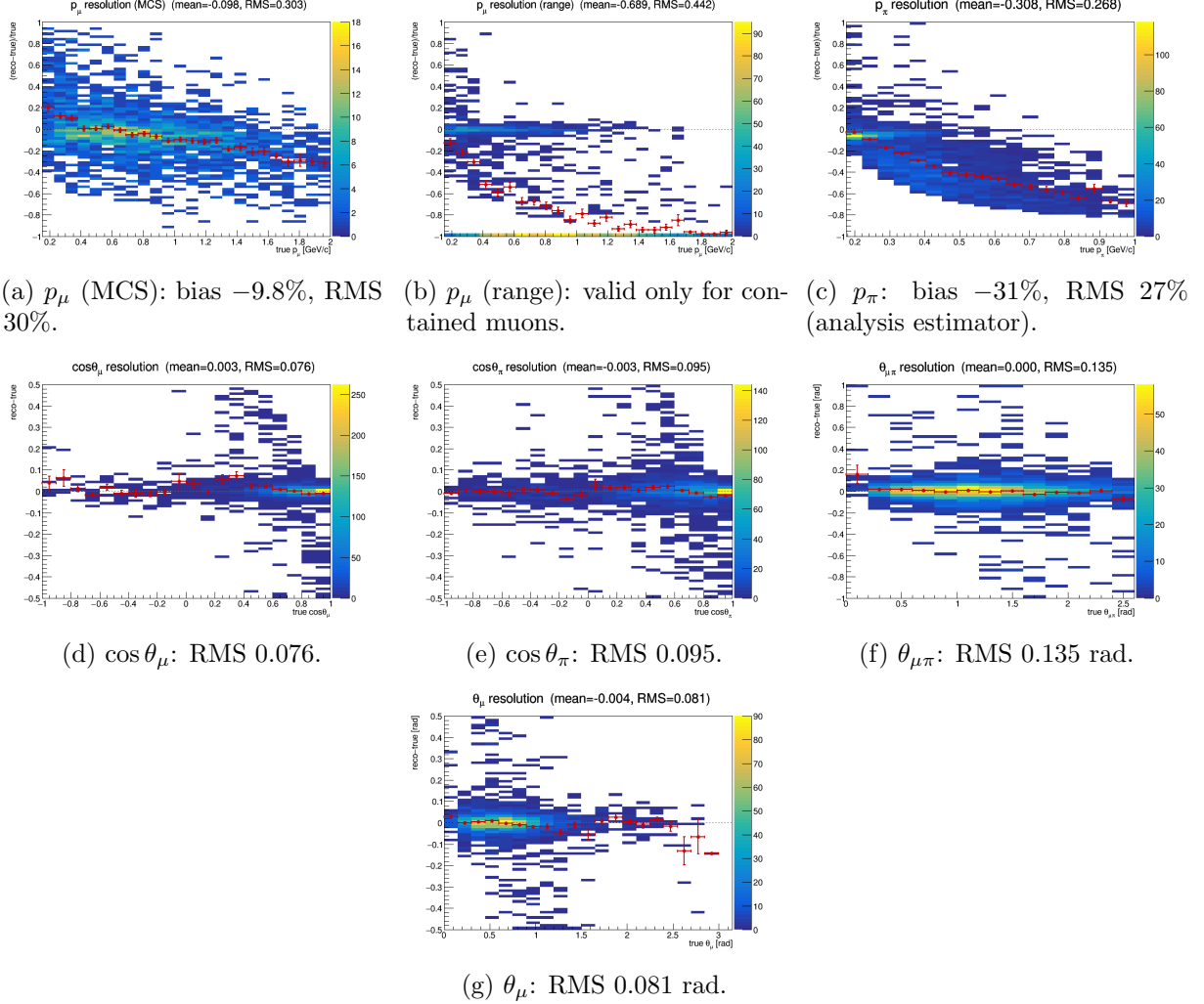
Figure 19: Reconstruction resolution vs. true value, selected signal. Momenta: relative (\text{reco} - \text{true})/\text{true} ; angles: absolute (\text{reco} - \text{true}) . Red points: mean residual per true bin. \theta_\mu is derived as \arccos(\cos\theta_\mu) , exactly as the bin config does it, so the panel shows the quantity the analysis bins on; it is unbiased ( -0.004 rad) with RMS 0.081 rad, the drift below zero above \sim 2.5 rad being a handful of backward-going muons. The muon MCS momentum slightly over-estimates at low p_\mu and increasingly under-estimates above \sim 1 GeV/c; the range estimator is badly biased for exiting muons (range = distance to wall), which is why the analysis uses range only for contained muons (range-or-MCS). The pion panel shows the estimator the analysis actually bins on, not the raw candidate_pion_mom_reco branch (§8.8): mean bias -31\% , RMS 27\% . That average is dominated by high momenta; the bias is only -2\% in the first true bin and reaches -65\% above 0.8 GeV/c; because the reconstructed value saturates near 0.34 GeV/c once pions interact hadronically before stopping. The angular variables are essentially unbiased with narrow resolution.
