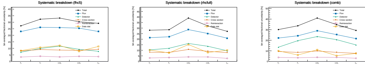
Figure 30: Bin-averaged fractional systematic uncertainty by source vs. observable, for FHC (left), RHC (centre) and combined (right); the figure form of Tables 30–32. Colours use the Okabe-Ito colourblind-safe palette with distinct markers per source: total (black), flux (blue), detector (green), cross section (vermillion), reinteraction (purple), data stat (orange).
