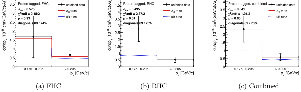
Figure 23: The two-bin p_\pi cross section on the proton-tagged CC1mu1pi1p selection, the graphical form of Tab. 16. Same edges as the inclusive result of Fig. 21 so the two are directly comparable, and the bins are again drawn equal-width.
